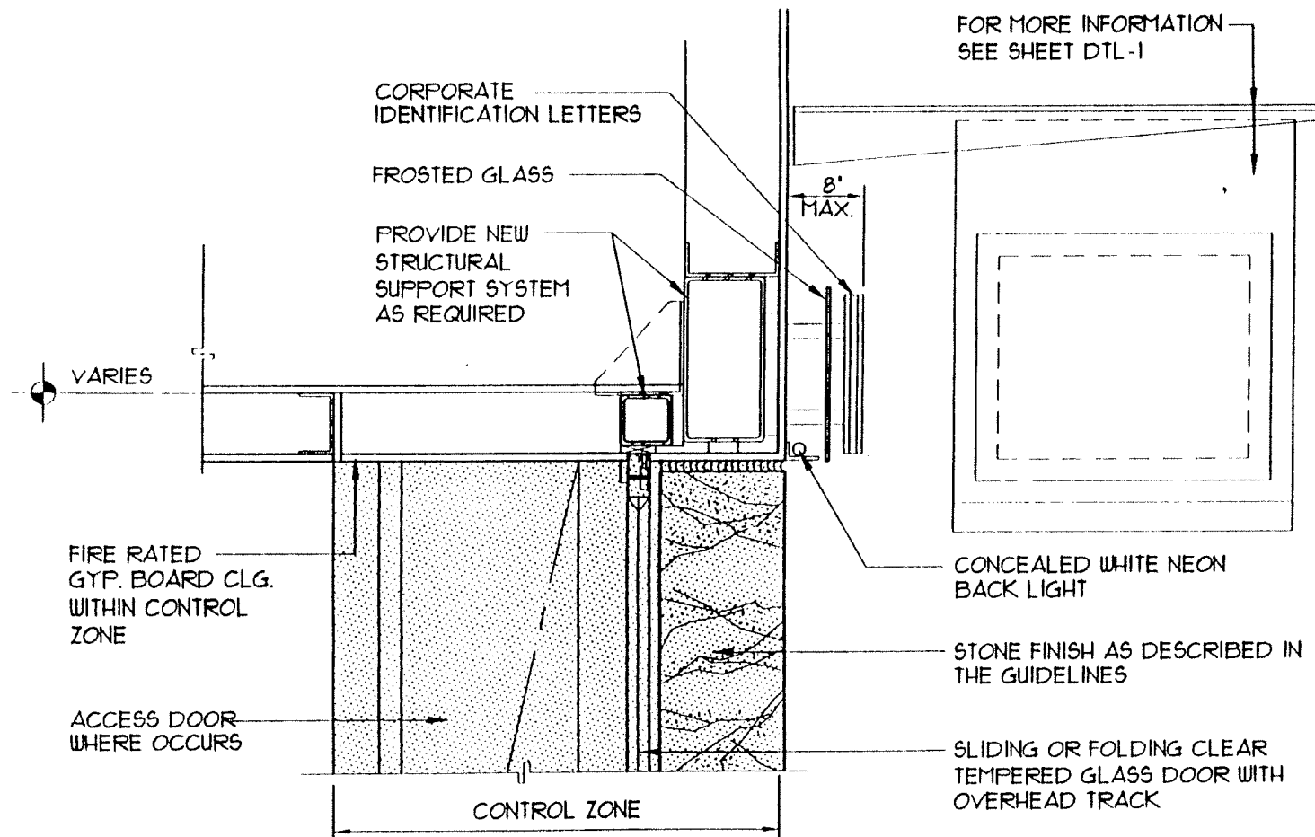
SOFFIT DETAIL - CONDITION #1
