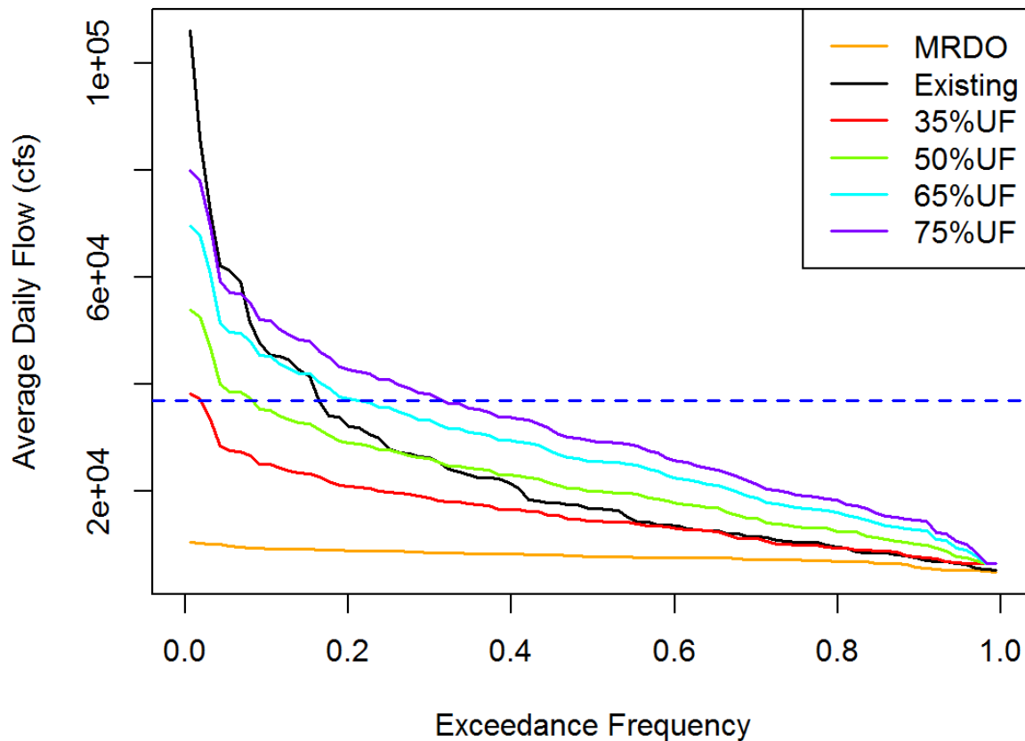
Figure 5.3-9. Frequency of Meeting March-July Delta Outflows to Benefit White and Green Sturgeon for Minimum Required Delta Outflow (MRDO), Existing Conditions as Modeled by CalSim II, and Delta Outflows Resulting from 35% to 75% of Unimpaired Delta Inflow.
