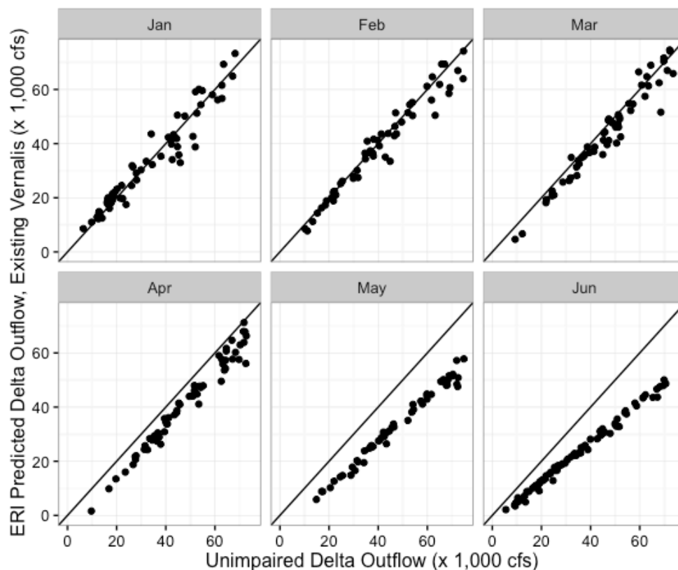
Figure 5.3-2. Predicted Delta Outflow as a Function of ERI, Assuming Existing Condition Flows at Vernalis. April-June flows generally fall below the one-to-one line due to the impairment of Vernalis flows.
