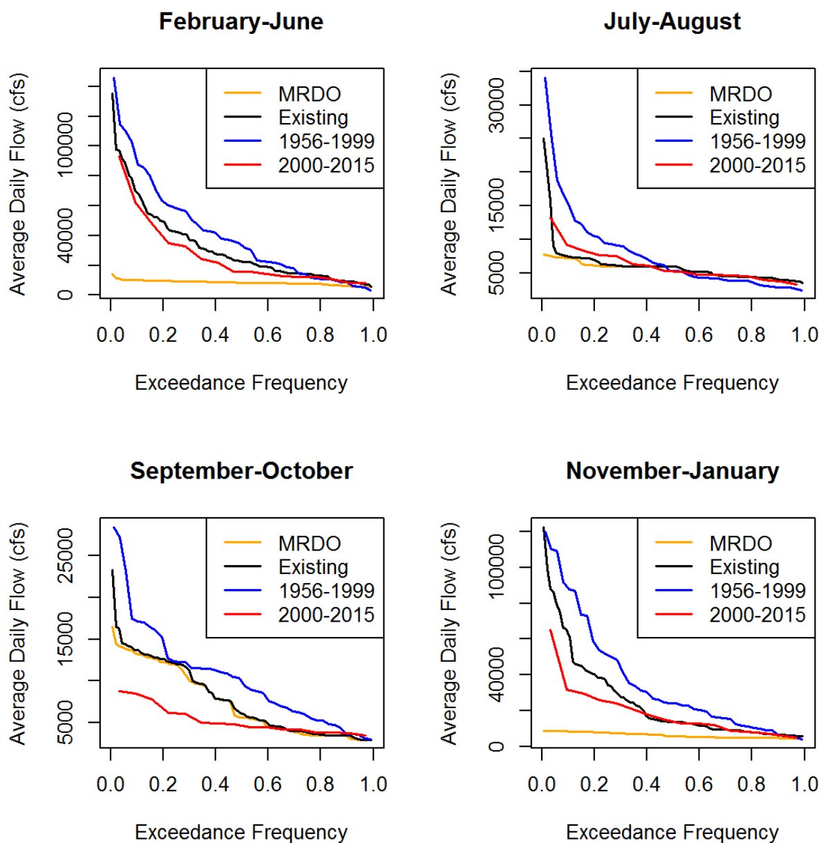
Figure 5.3-3. Comparison of Minimum Required Delta Outflow (“MRDO”, orange line), CalSim II Modeled Delta Outflow (“Existing”, black line), and Observed Delta Outflow for 1956-1999 (blue) and 2000-2015 (red) (Dayflow data, DWR 2016).
