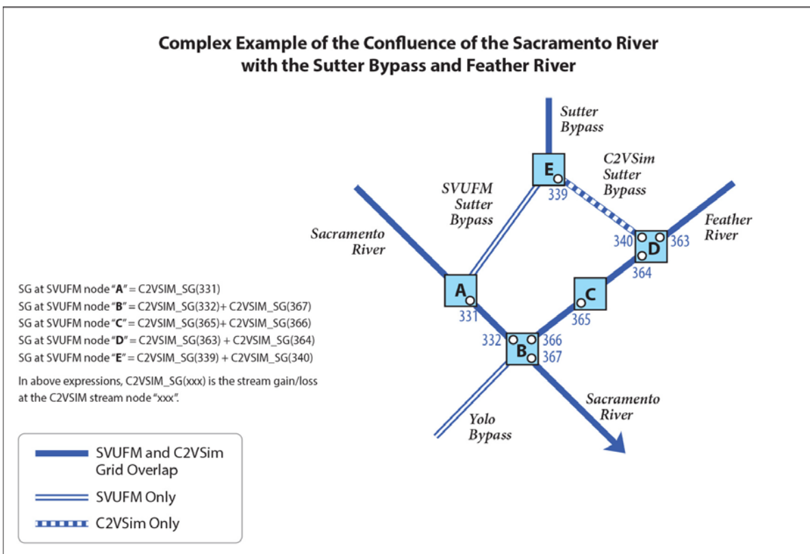
Figure A-4. Assignment of C2VSim Stream-Groundwater Interaction to SVUFM Nodes
