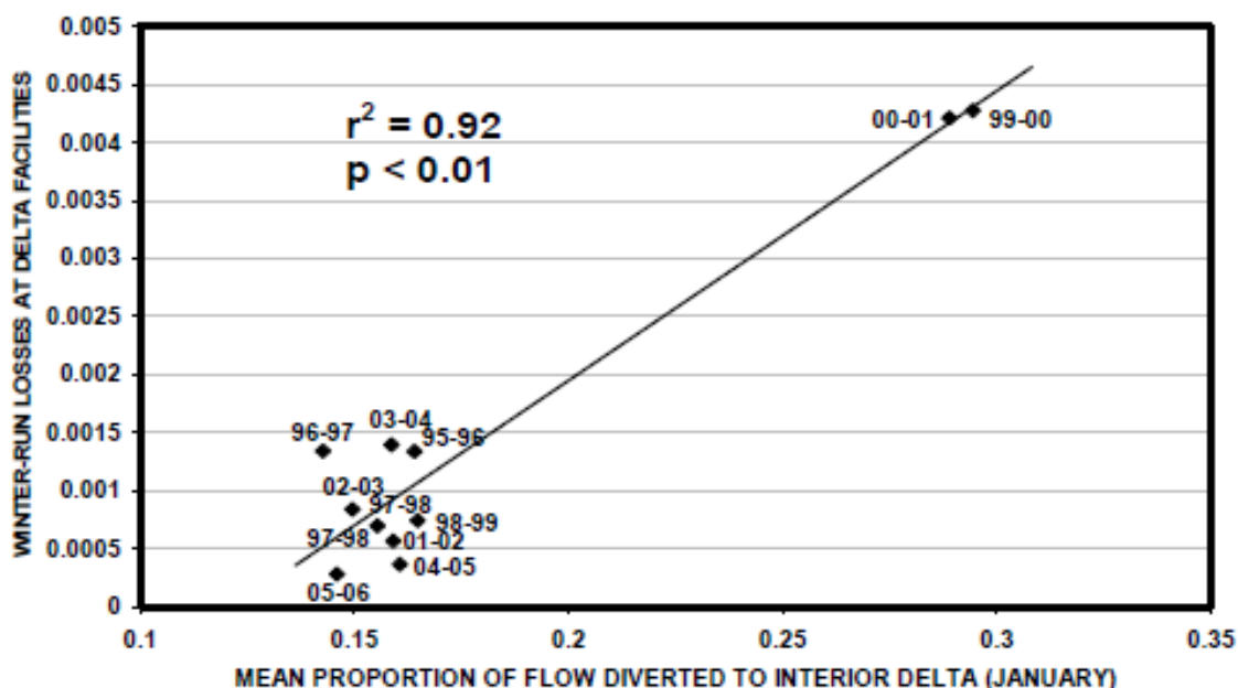
Figure 3.4-13. Relationship between the Mean Proportion of Flow Diverted into the Interior Delta in January and the Proportion of Juvenile Winter-run Lost at the CVP and SWP Pumping Facilities (loses divided by the juvenile production index) October 1 through May 31, 1996-2006 (from Low and White, 2006).
