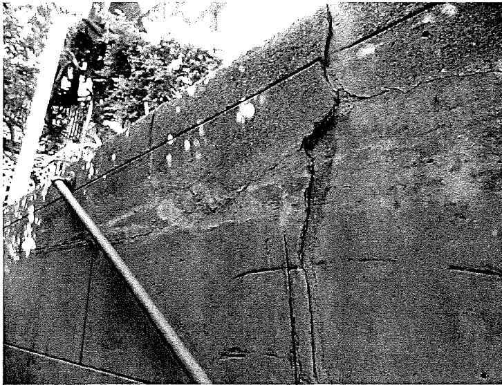
Figure 16. Cracked retaining wall along east property line. (Photograph by Garavaglia Architecture, Inc., April 2015.)
