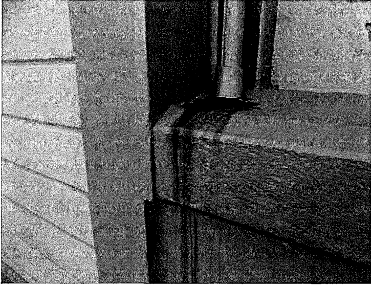
Figure 22. Corroded downspout along north elevation. (Photograph by Garavaglia Architecture, Inc., April 2015.)
