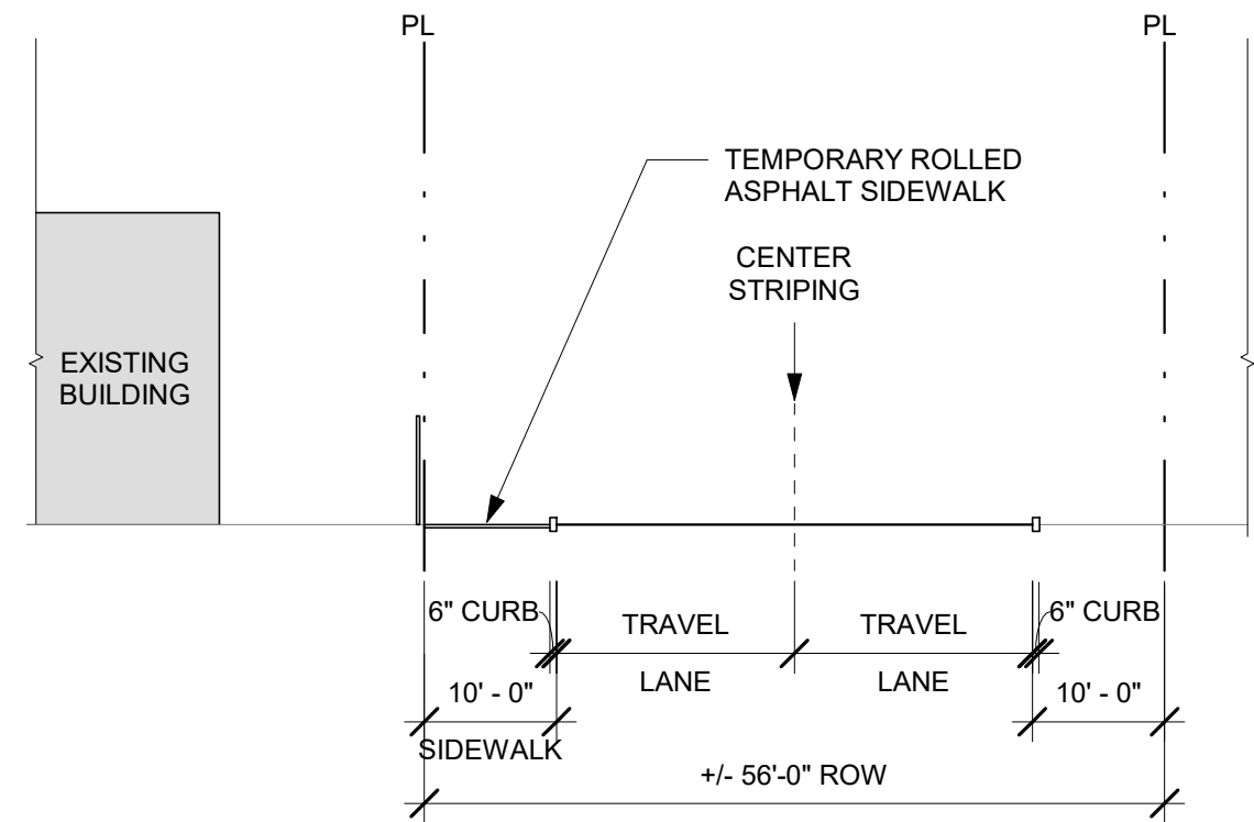
1 STREET SECTION AT INNES EXTENSION 1/16" = 1'-0"
