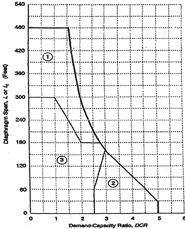
FIGURE 5C-1 – ACCEPTABLE DIAPHRAGM SPAN
