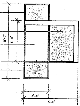
TOP VIEW (WITH SUNSHADES OPEN)
