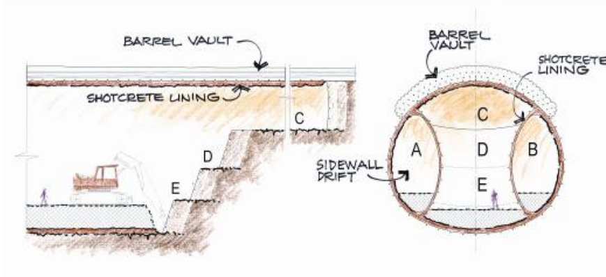
FIGURE 6-3 TUNNEL CONSTRUCTION USING SEQUENTIAL EXCAVATION METHOD (SEM)
