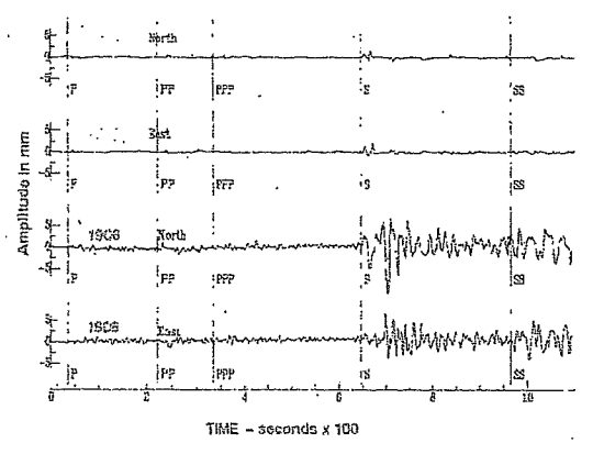
Comparison of 1906 and Loma Prieta records at Gottingen, Germany
