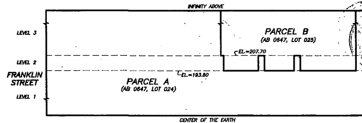
SECTION "A"
