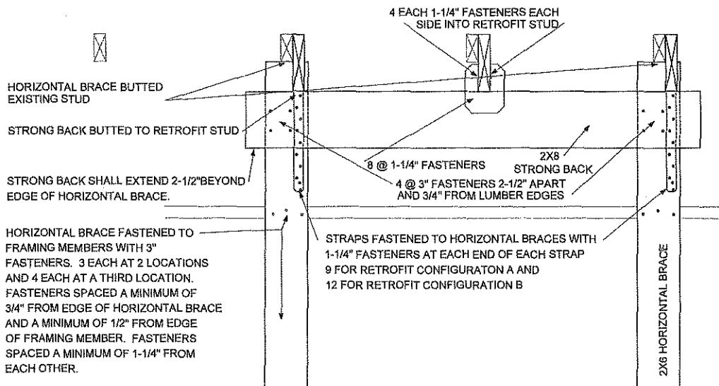
[BS] FIGURE C104.2.3 OMITTED HORIZONTAL BRACE
