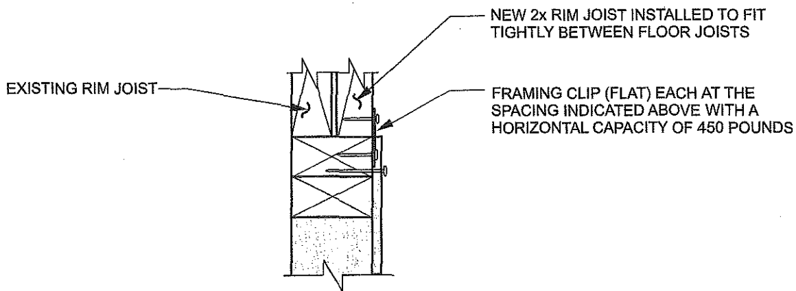
ALTERNATIVE CONNECTION FOR FLUSH CONNECTION
