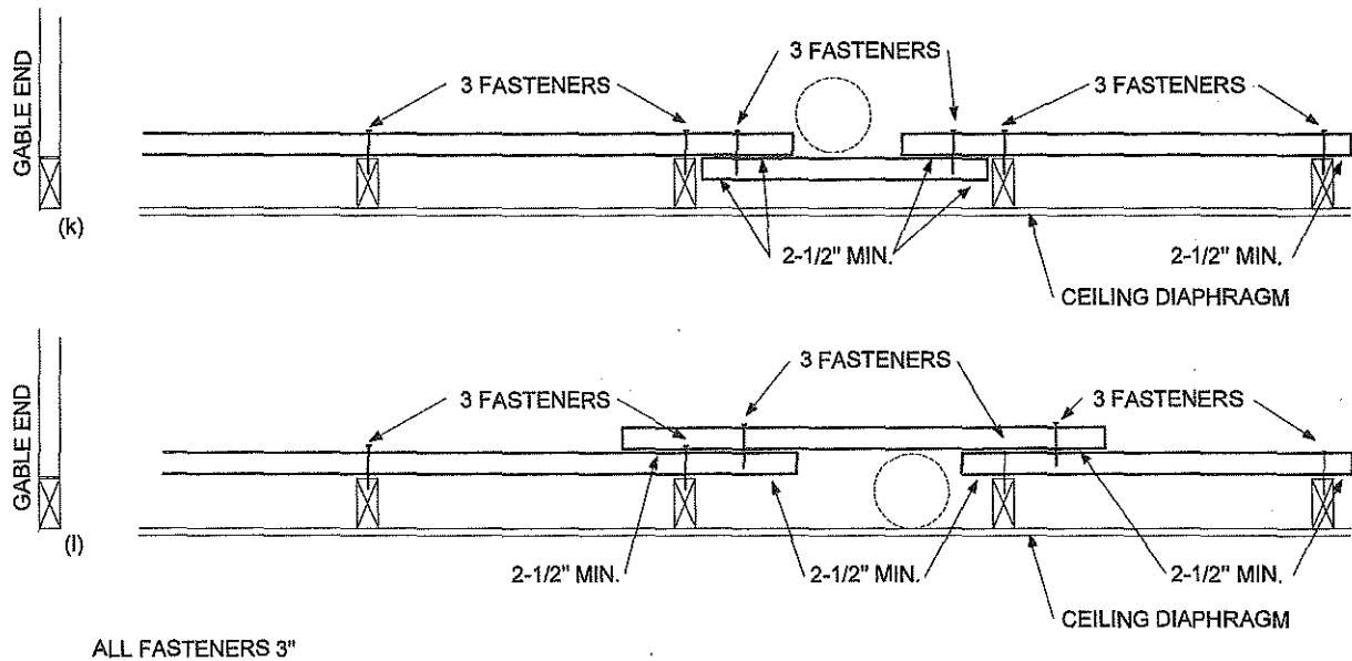
[BS] FIGURE C104.2.8(3) SPLICED HORIZONTAL BRACES
