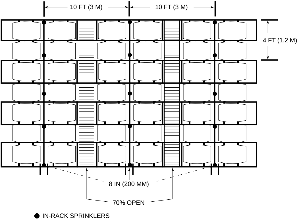
FIGURE 4005.2.3.6(1)—IN-RACK SPRINKLER LAYOUT FOR WOODEN BARRELS ON THEIR SIDES (PLAN VIEW)
