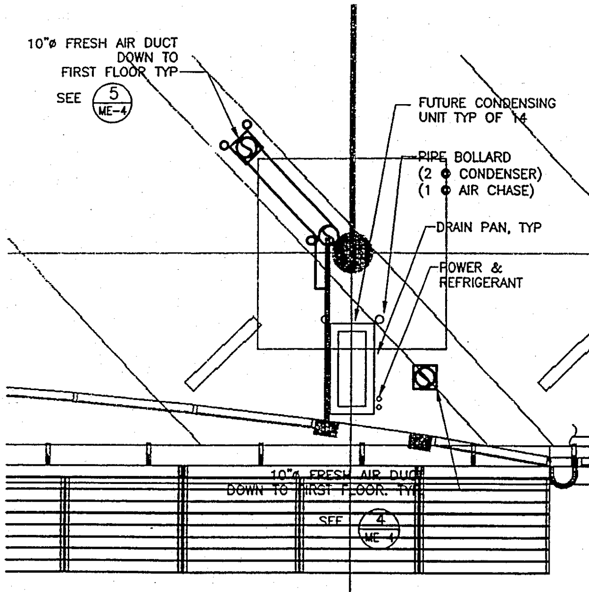
TYPICAL MECHANICAL / ELECTRICAL LAYOUT ON 2 ND FLOOR
