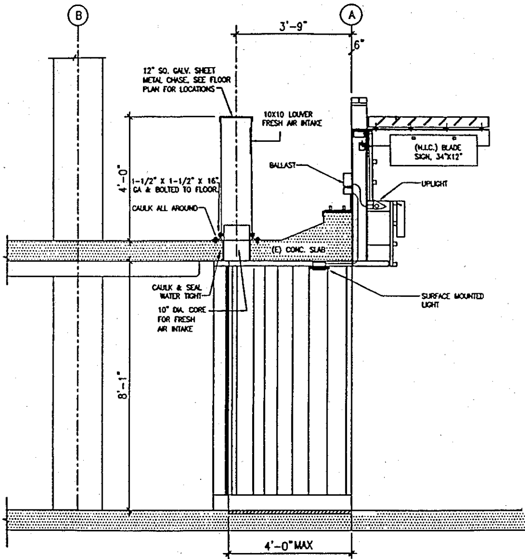
4/ME-4 MECHANICAL / ELECTRICAL DETAIL
