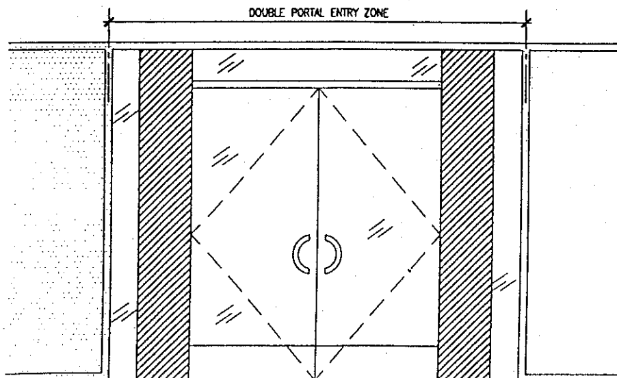
PORTAL ELEVATIONS
