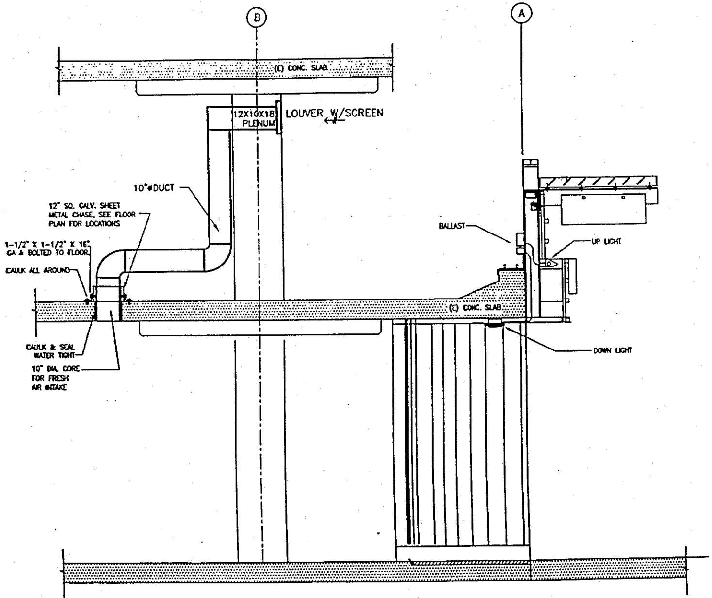
5/ME-5 MECHANICAL / ELECTRICAL DETAIL
