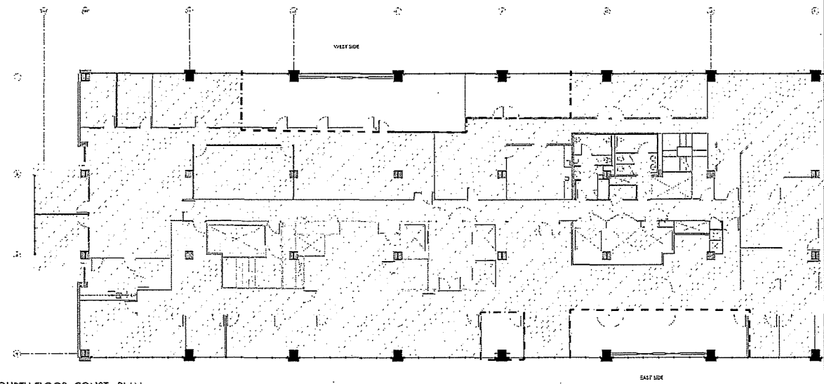
FOURTH FLOOR CONST. PLAN
