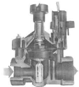
PESB Cutaway
