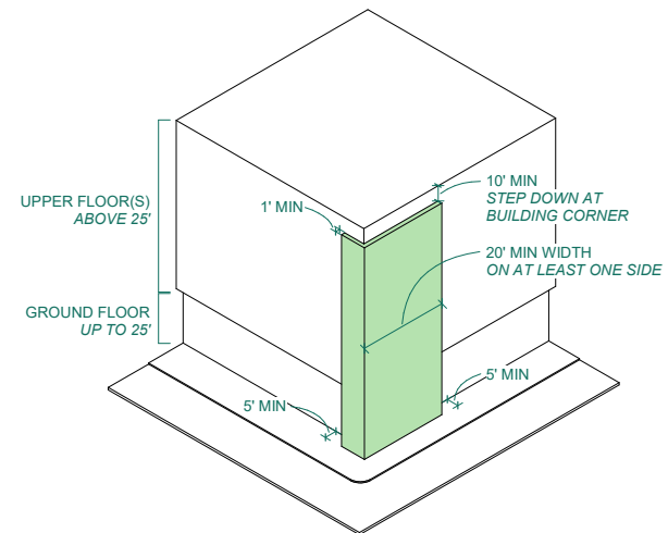
Figure S.3.2A - Corner Variation Element
