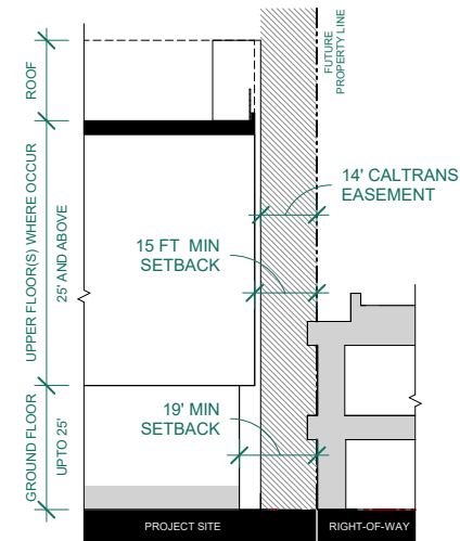
Figure S.2.1A Selby Street Setbacks
