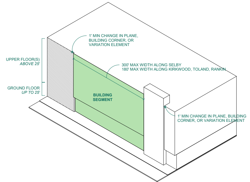
Figure S.3.1A Building Segment
