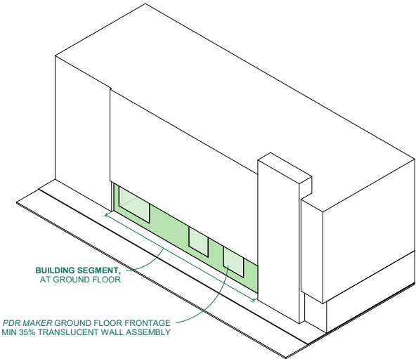
Figure S.6.2C - Ground Floor Translucency at PDR Maker Frontage
