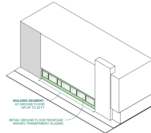
Figure S.6.3A - Ground Floor Transparent Glazing at Retail Frontage
