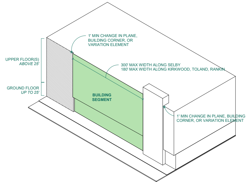
Figure S.3.1A Building Segment
