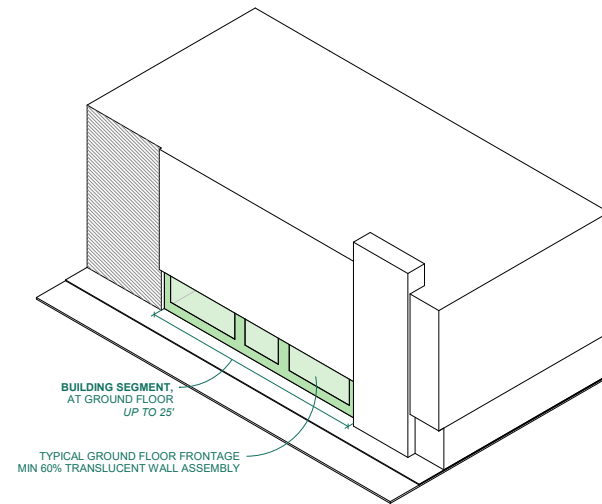
Figure S.6.2A - Typical Ground Floor Translucency
