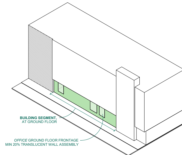
Figure S.6.2B - Ground Floor Translucency at Office Frontage
