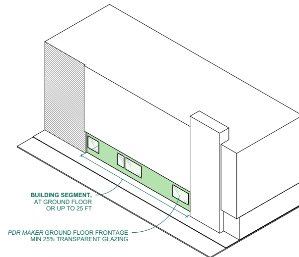
Figure S.6.3C - Ground Floor Transparent Glazing at PDR Maker Frontage
