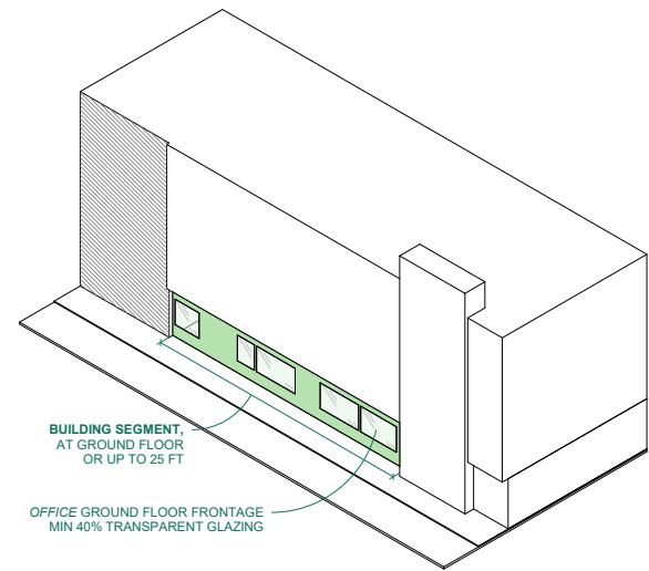
Figure S.6.3B - Ground Floor Transparent Glazing at Accessory Office Frontage
