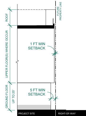
Figure S.2.1B Typical Setbacks
