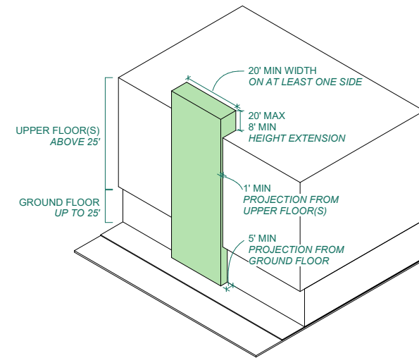
Figure S.3.2A - Typical Variation Element
