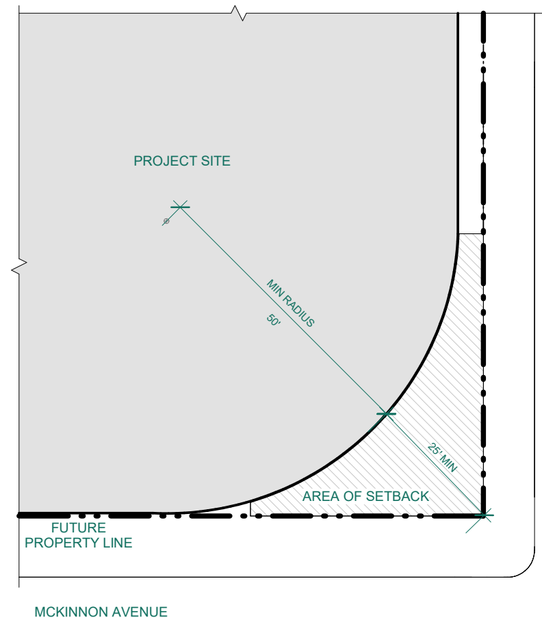
Figure S.2.3C McKinnon Avenue Intersection Setback
