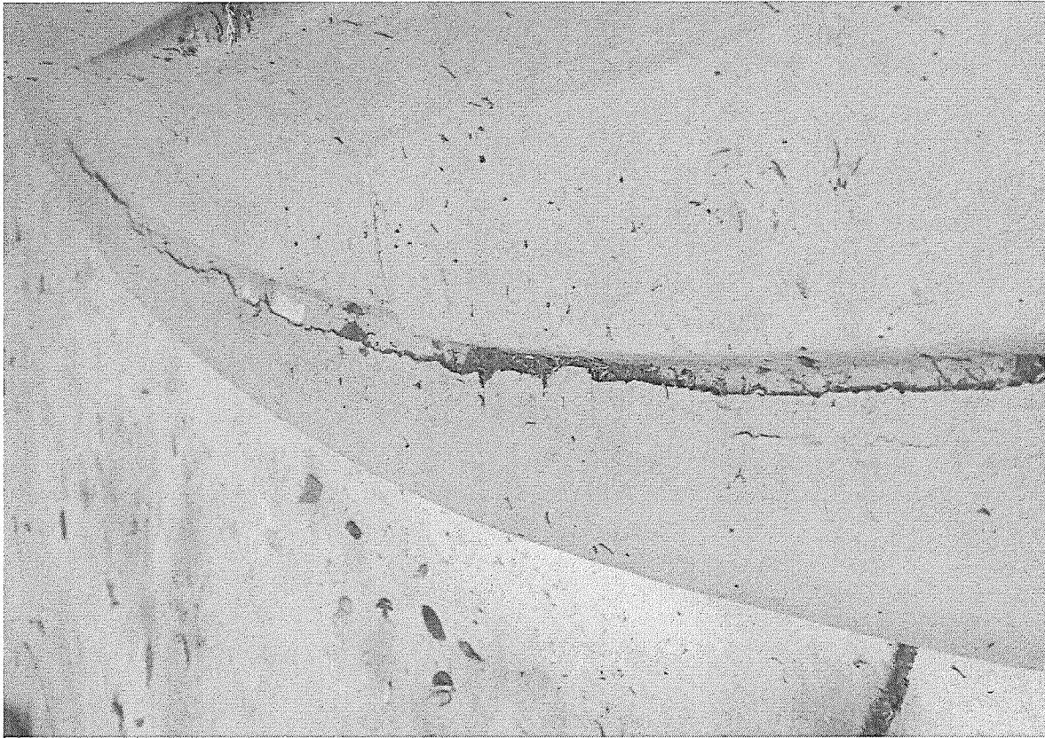
Figure 28: Detail of area where soft deteriorated wood was noted with moisture at the wood.
