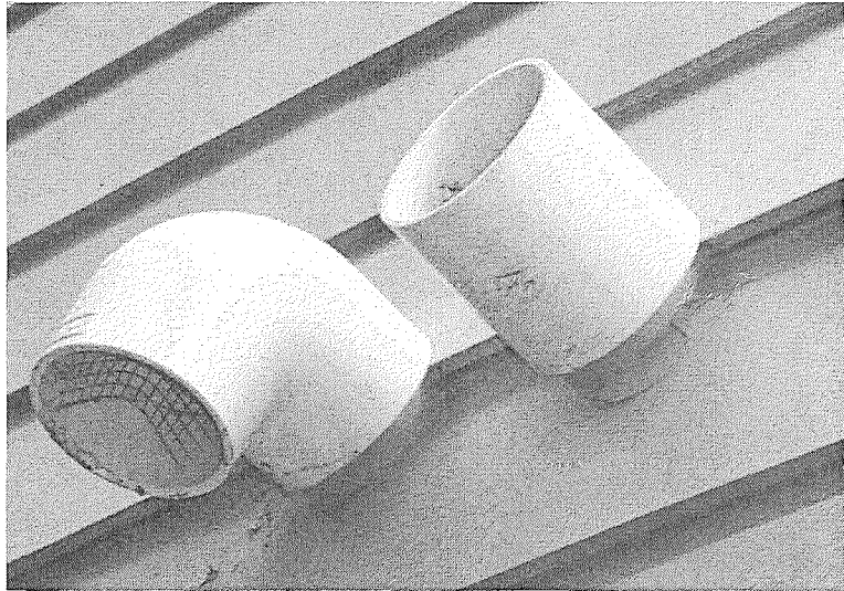
Figure 33: Detail of damaged siding beneath vent.
