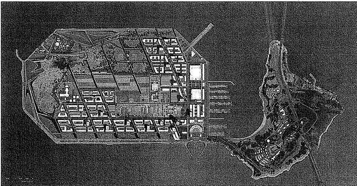
Illustrative Conceptual Land Plan
