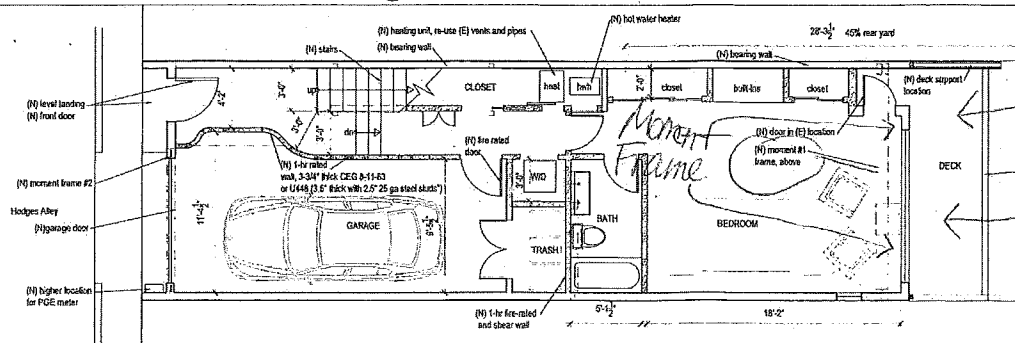
PROPOSED GROUND FLOOR PLAN 1/4" = 1'-0"
