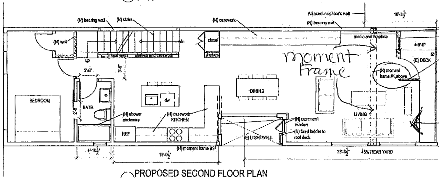
PROPOSED SECOND FLOOR PLAN 1/4" = 1'-0"
