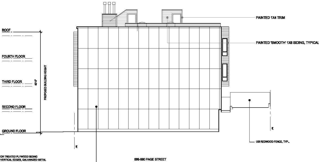
686-690 PAGE STREET EAST ELEVATION
