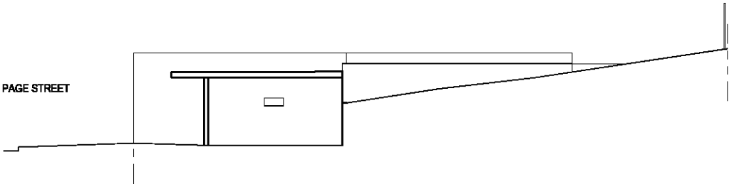
690 PAGE STREET/EAST ELEVATIONS
