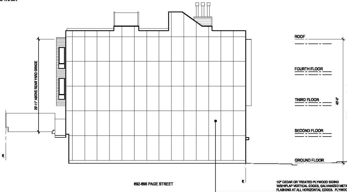
692-696 PAGE STREET WEST ELEVATION
