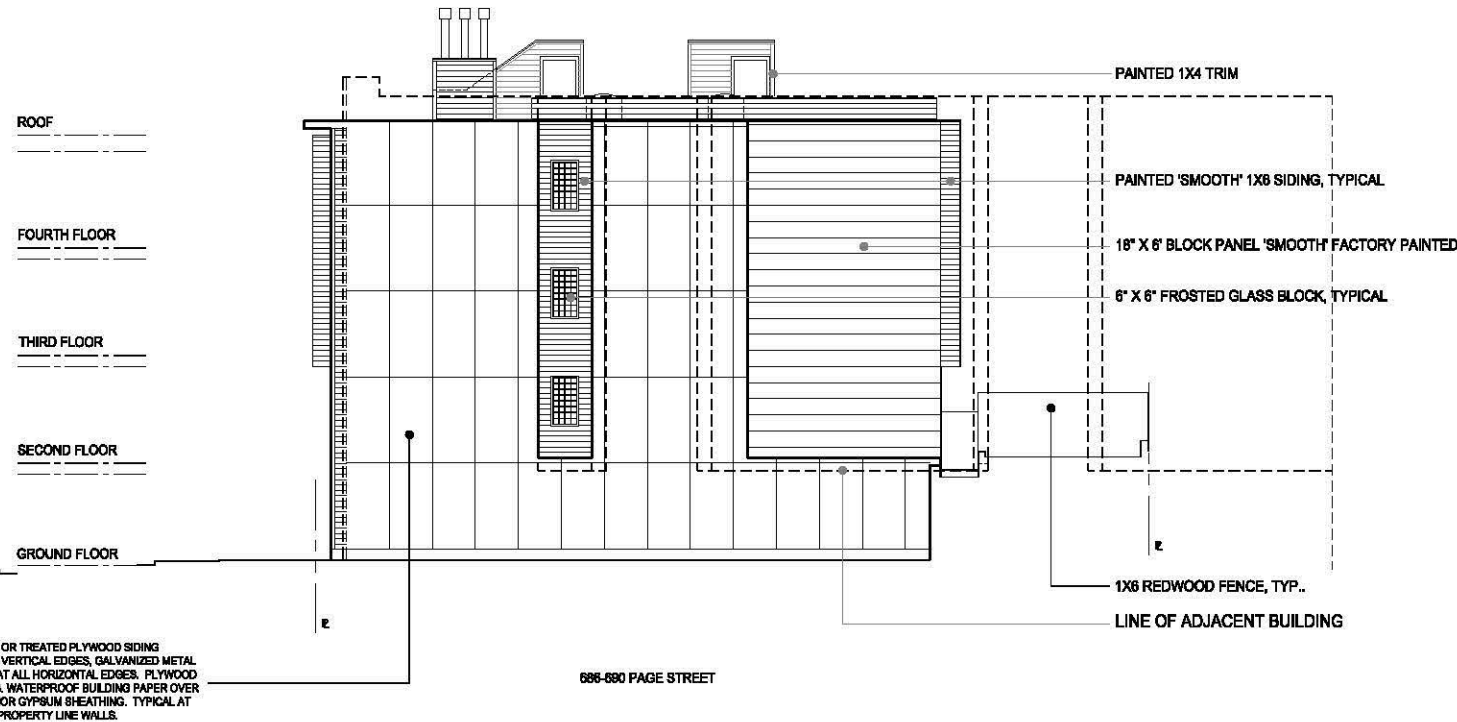
680-684 PAGE STREET EAST ELEVATION
