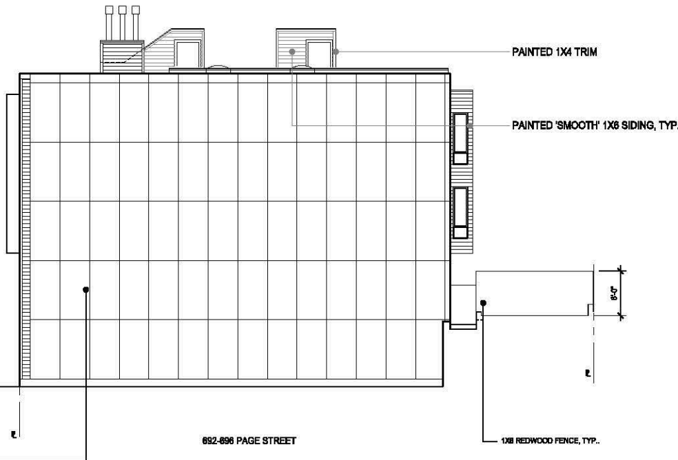
692-696 PAGE STREET EAST ELEVATION
