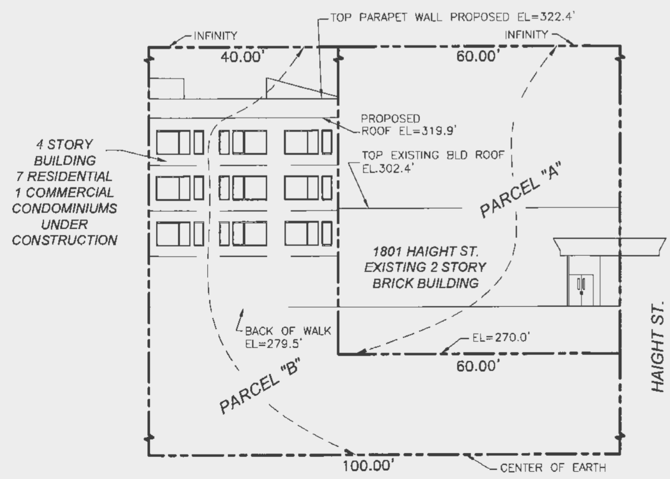
ELEVATION VIEW
