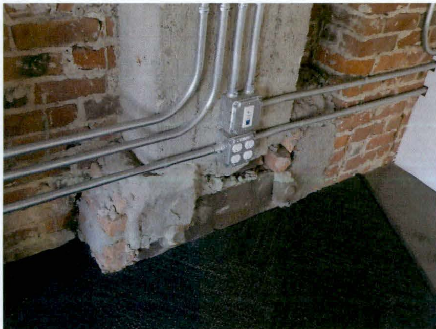
Photo Y: Detail of brick masonry at concrete walls at 3 rd level with exposed steel members and deteriorated mortar joints.
