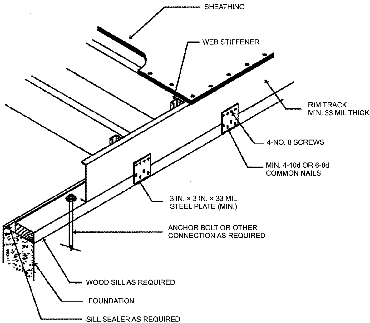
FIGURE R505.3.1(2) FLOOR TO WOOD SILL CONNECTION
