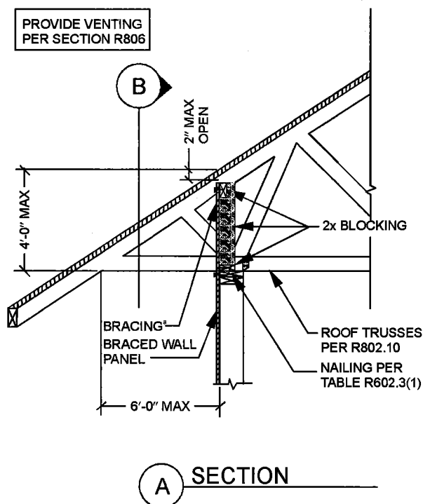
FIGURE R602.10.8.2(3) BRACED WALL PANEL CONNECTION OPTION TO PERPENDICULAR RAFTERS OR ROOF TRUSSES
