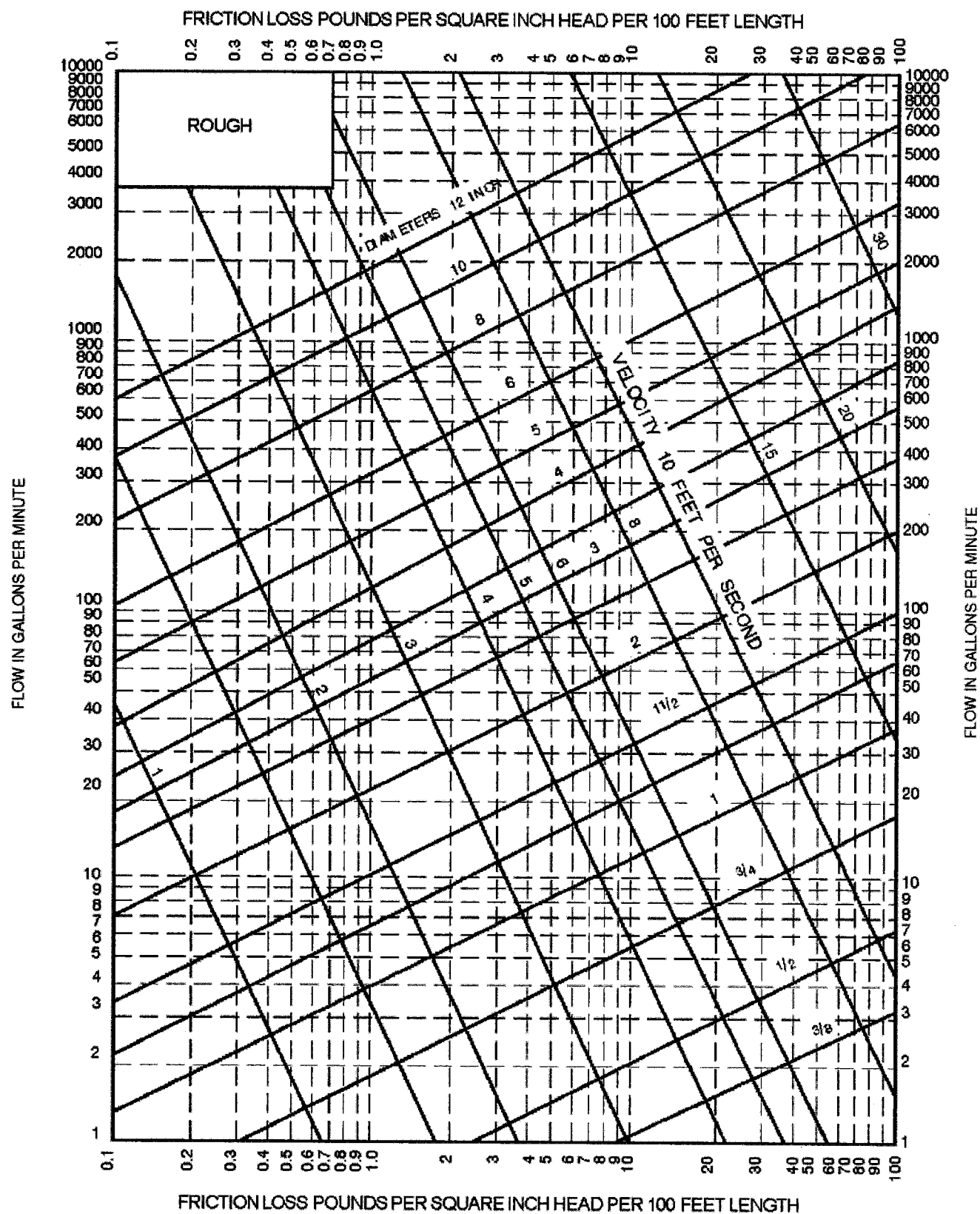
FIGURE AP103.3(7) FRICTION LOSS IN ROUGH PIPE*
