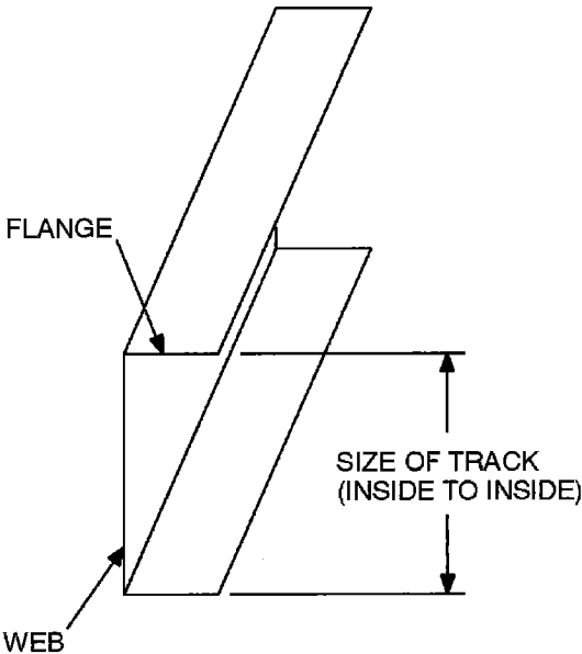
FIGURE R804.2(2) TRACK SECTION
