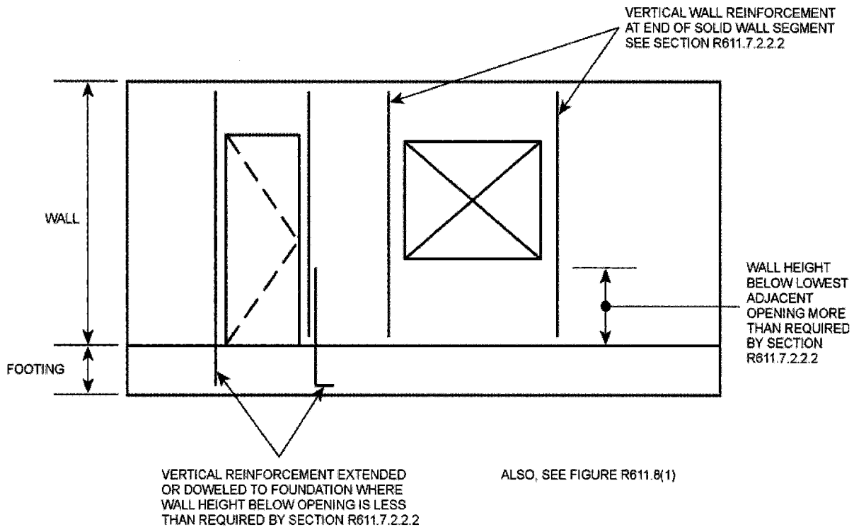
FIGURE R611.7(3) VERTICAL WALL REINFORCEMENT ADJACENT TO WALL OPENINGS
