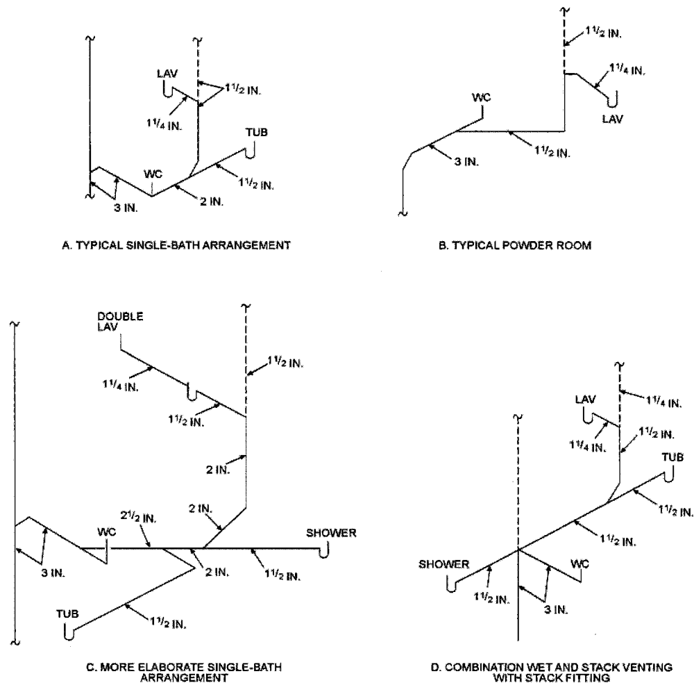
FIGURE N1 TYPICAL SINGLE-BATH WET-VENT ARRANGEMENTS
