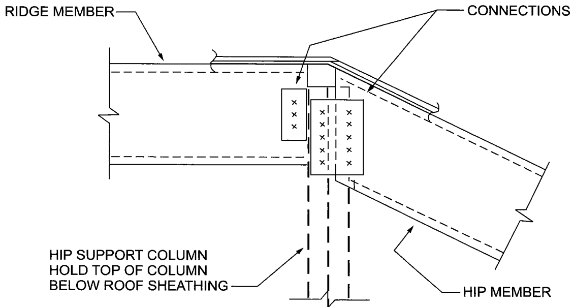
FIGURE R804.3.3.4(3) HIP CONNECTIONS AT RIDGE
