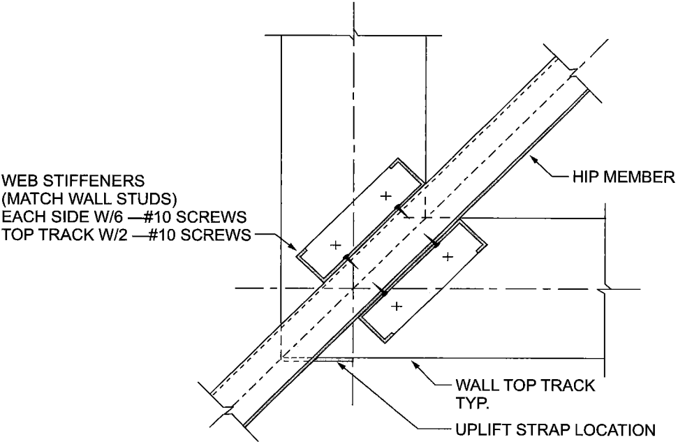
FIGURE R804.3.3.4(5) HIP MEMBER CONNECTION AT WALL CORNER
