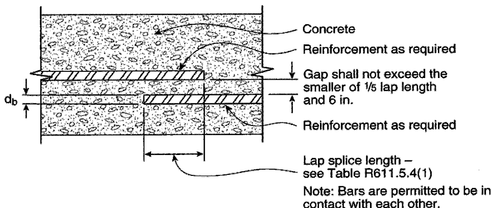
FIGURE R611.5.4(1) LAP SPLICES
