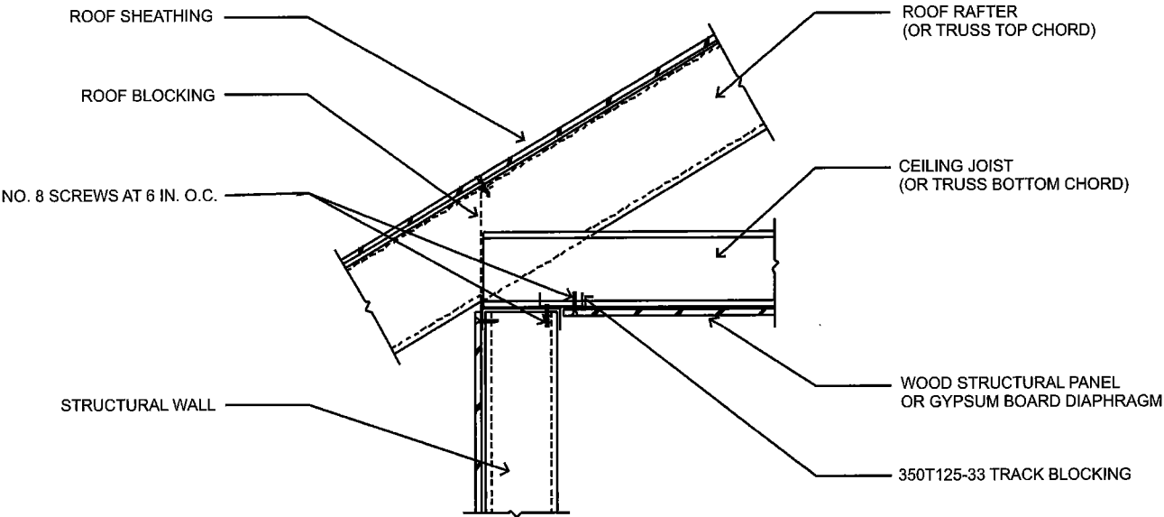
FIGURE R804.3.8(2) CEILING DIAPHRAGM TO SIDEWALL DETAIL
