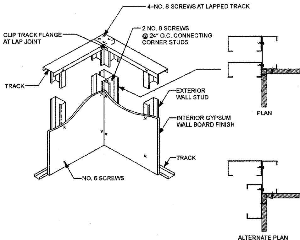
FIGURE R603.4 CORNER FRAMING
