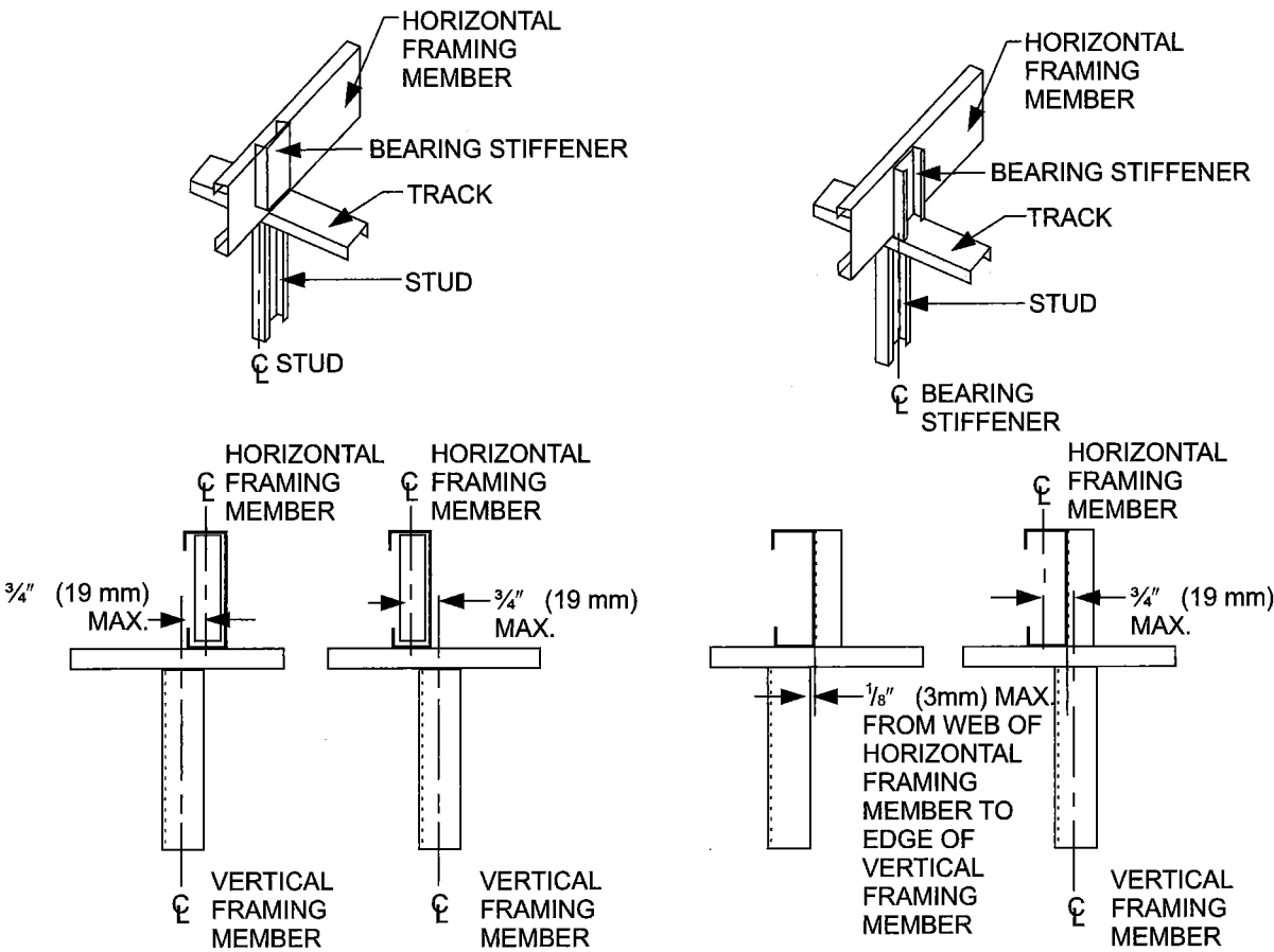
FIGURE R505.1.2 IN-LINE FRAMING
