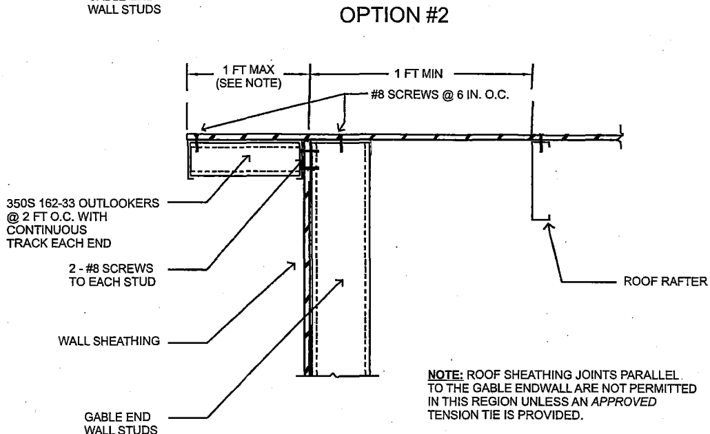
FIGURE R804.3.2.1.2 GABLE ENDWALL OVERHANG DETAILS
