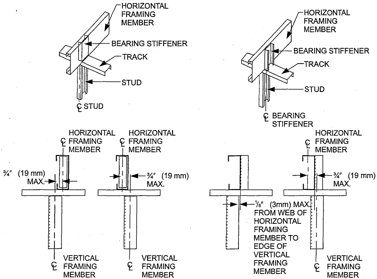
FIGURE R505.1.2 IN-LINE FRAMING
