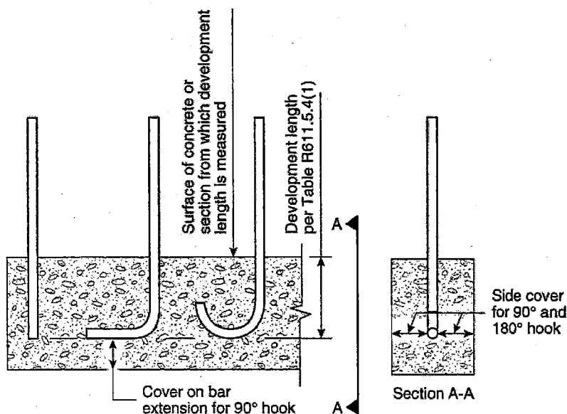
FIGURE R611.5.4(2) DEVELOPMENT LENGTH AND COVER FOR HOOKS AND BAR EXTENSION
