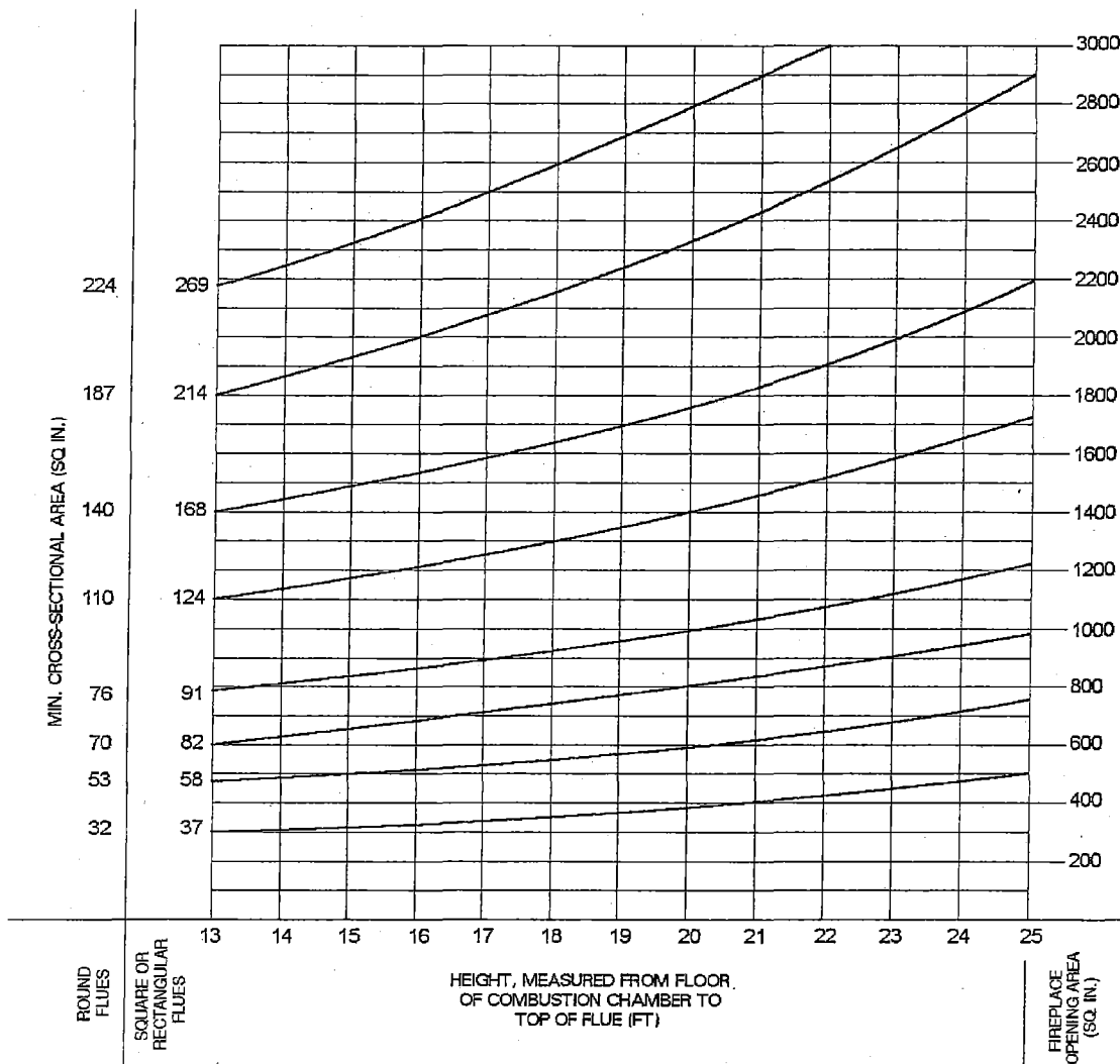
FIGURE R1003.15.2 FLUE SIZES FOR MASONRY CHIMNEYS
