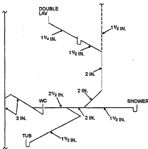
C. MORE ELABORATE SINGLE-BATH ARRANGEMENT
