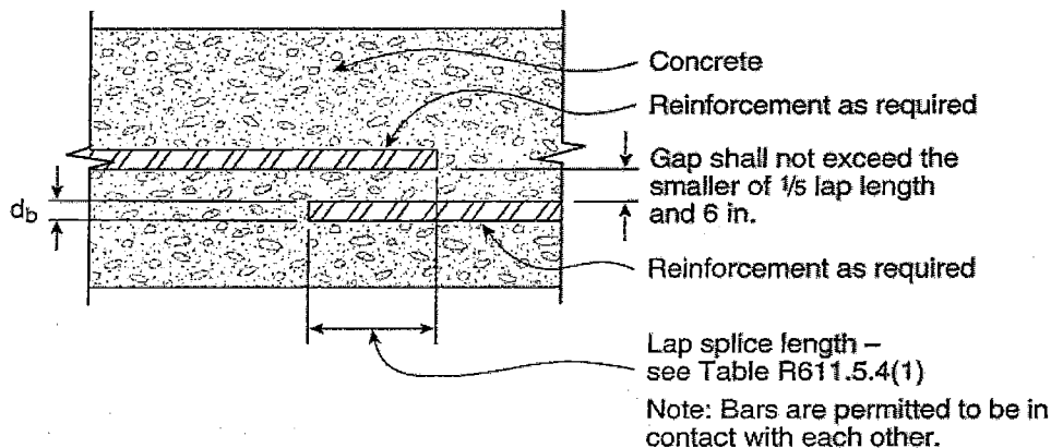
FIGURE R611.5.4(1) LAP SPLICES 2382
