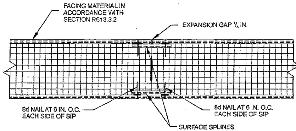
SURFACE SPLINE CONNECTION
