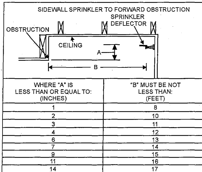
FIGURE R313.3.2.4.2 MINIMUM ALLOWABLE DISTANCE BETWEEN SPRINKLER AND OBSTRUCTION
