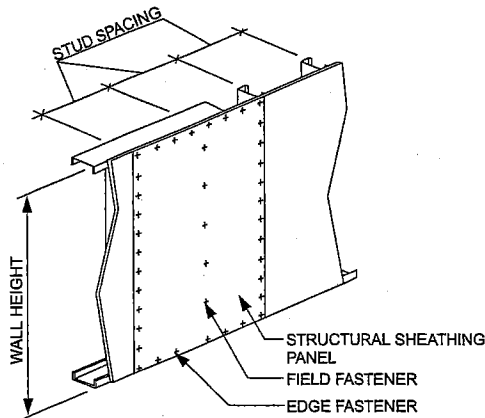
FIGURE R603.9 STRUCTURAL SHEATHING FASTENING PATTERN
