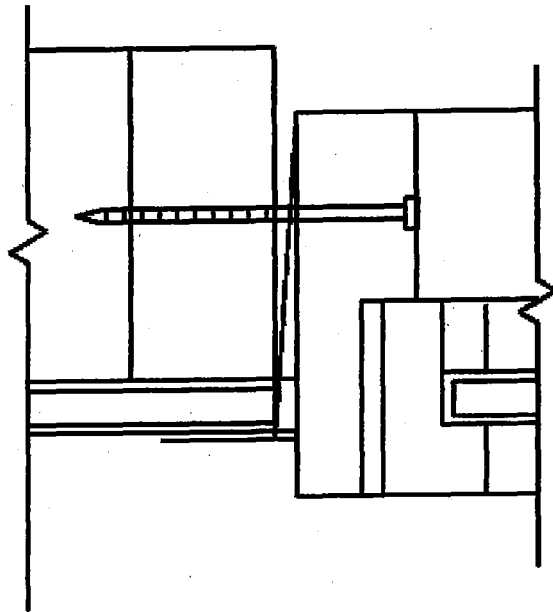
FIGURE R612.7.2(6) THROUGH THE FLANGE
