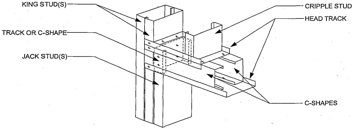
FIGURE R603.6.1(1) BOX BEAM HEADER IN GABLE ENDWALL
