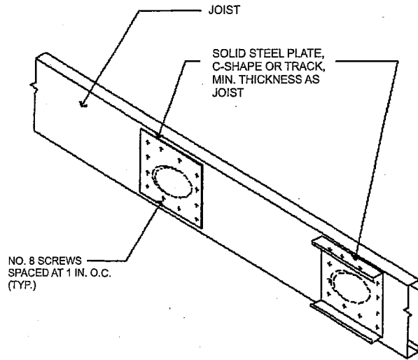
FIGURE R505.2.5.3 WEB HOLE PATCH
