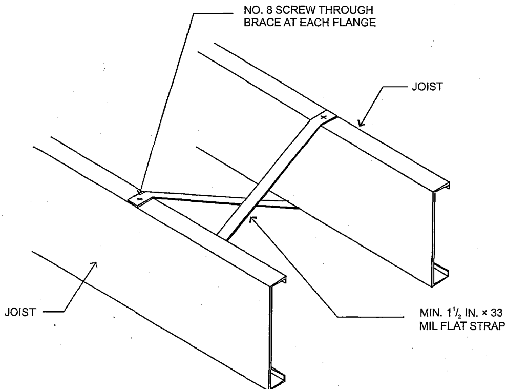
FIGURE R505.3.3.2(2) JOIST BLOCKING (STRAP) 2238
