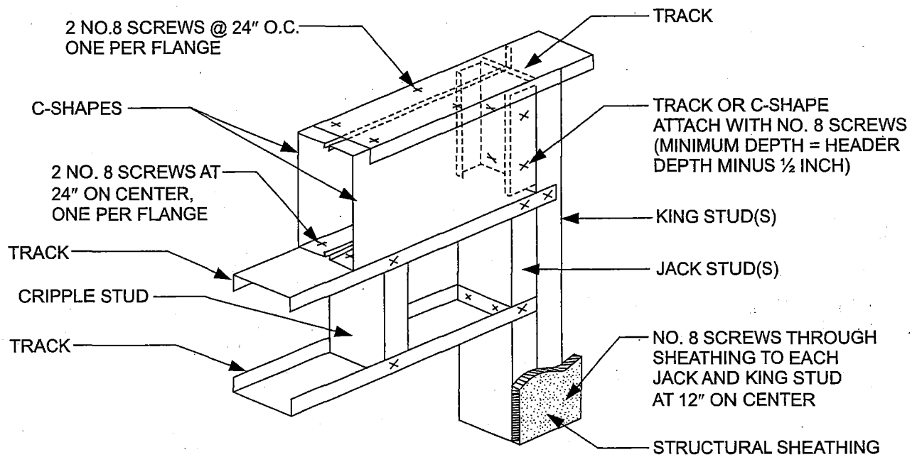
FIGURE R603.6(1) BOX BEAM HEADER
