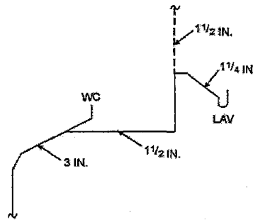
B. TYPICAL POWDER ROOM
