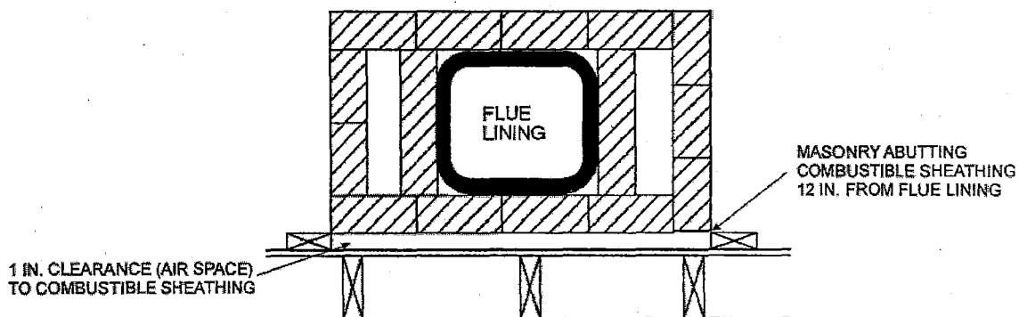
FIGURE R1003.18 CLEARANCE FROM COMBUSTIBLES 2563
