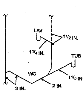
A. TYPICAL SINGLE-BATH ARRANGEMENT
