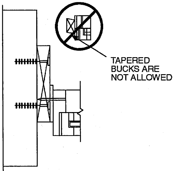
FIGURE R612.7.2(3) THROUGH THE FRAME
