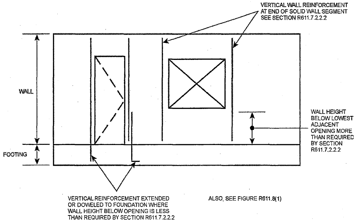
FIGURE R611.7(3) VERTICAL WALL REINFORCEMENT ADJACENT TO WALL OPENINGS
