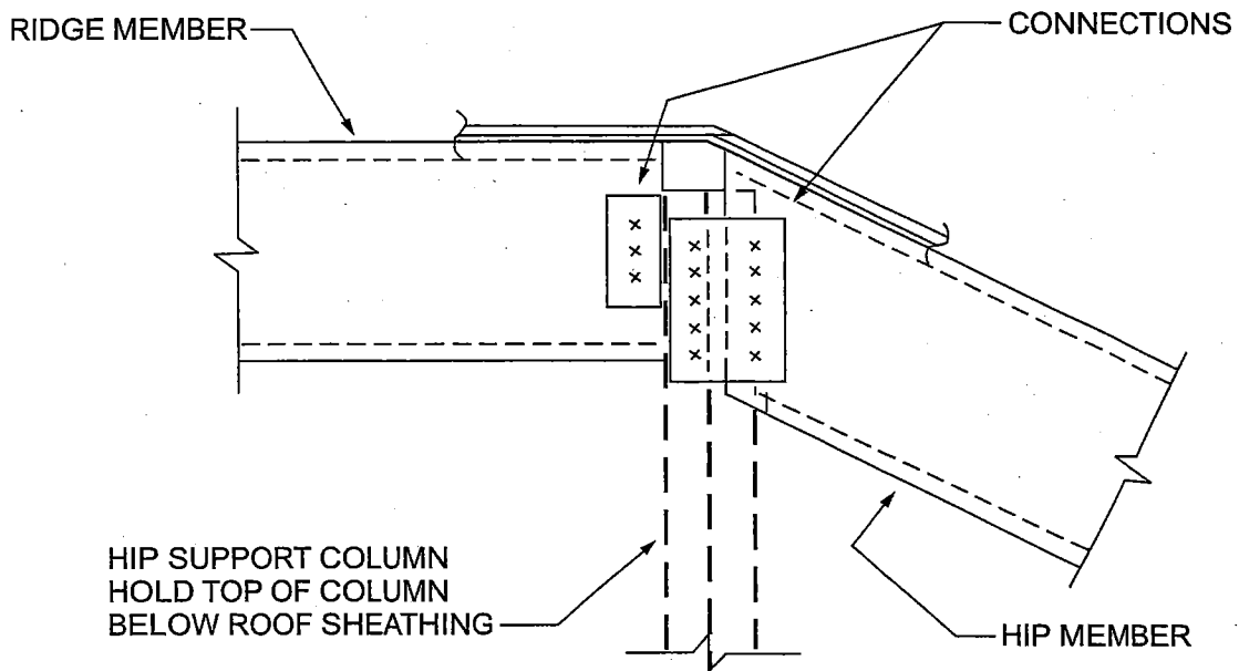
FIGURE R804.3.3.4(3) HIP CONNECTIONS AT RIDGE
