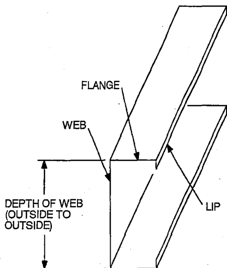
FIGURE R505.2(1) C-SHAPED SECTION
