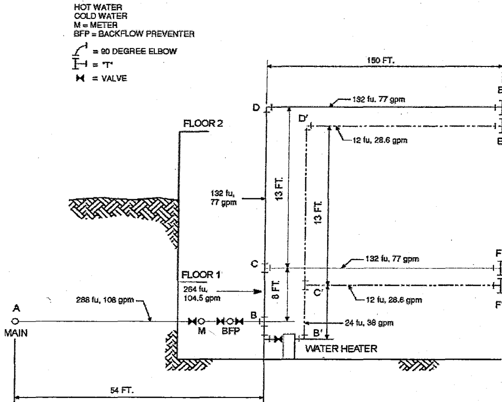
FIGURE AP103.3(1) EXAMPLE—SIZING
