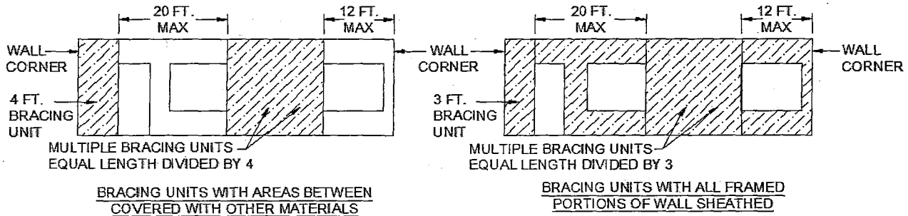
FIGURE R602.12.5 BRACING UNIT DISTRIBUTION
