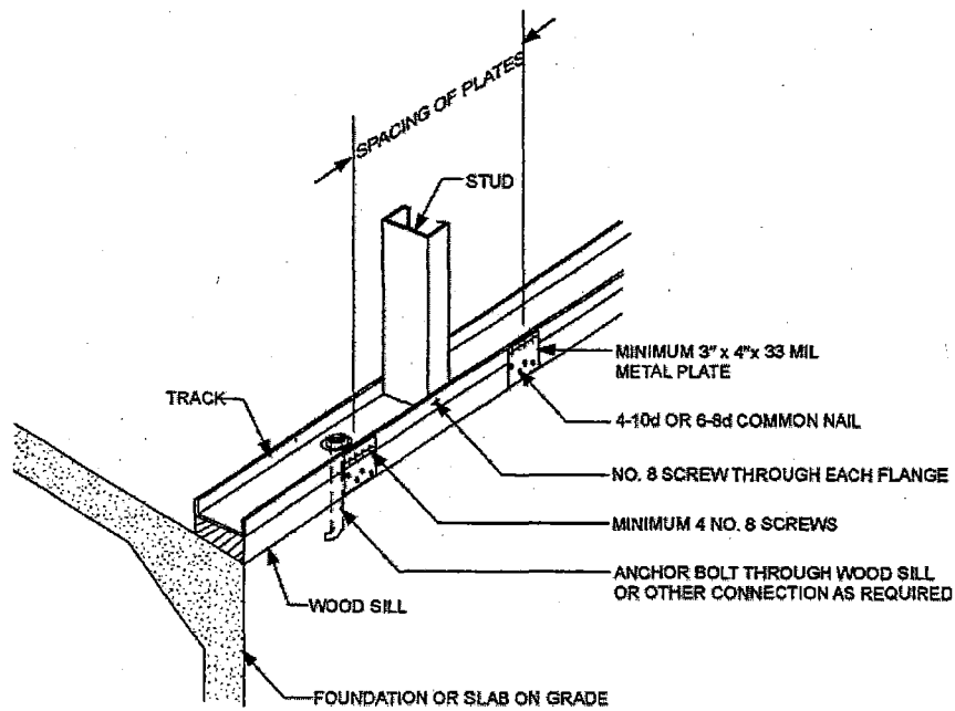
FIGURE R603.3.1(3) WALL TO WOOD SILL CONNECTION
