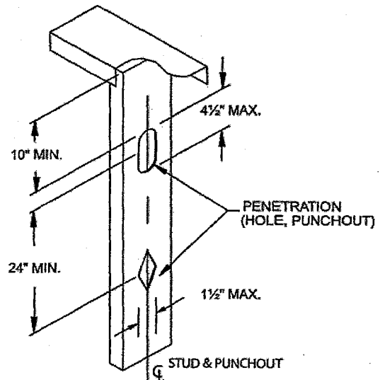
FIGURE R603.2.5.1 WEB HOLES
