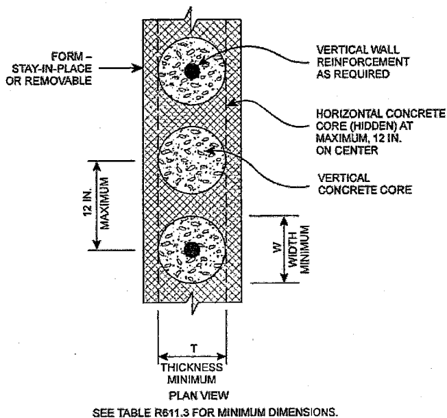
FIGURE R611.3(3) SCREEN-GRID WALL SYSTEM
