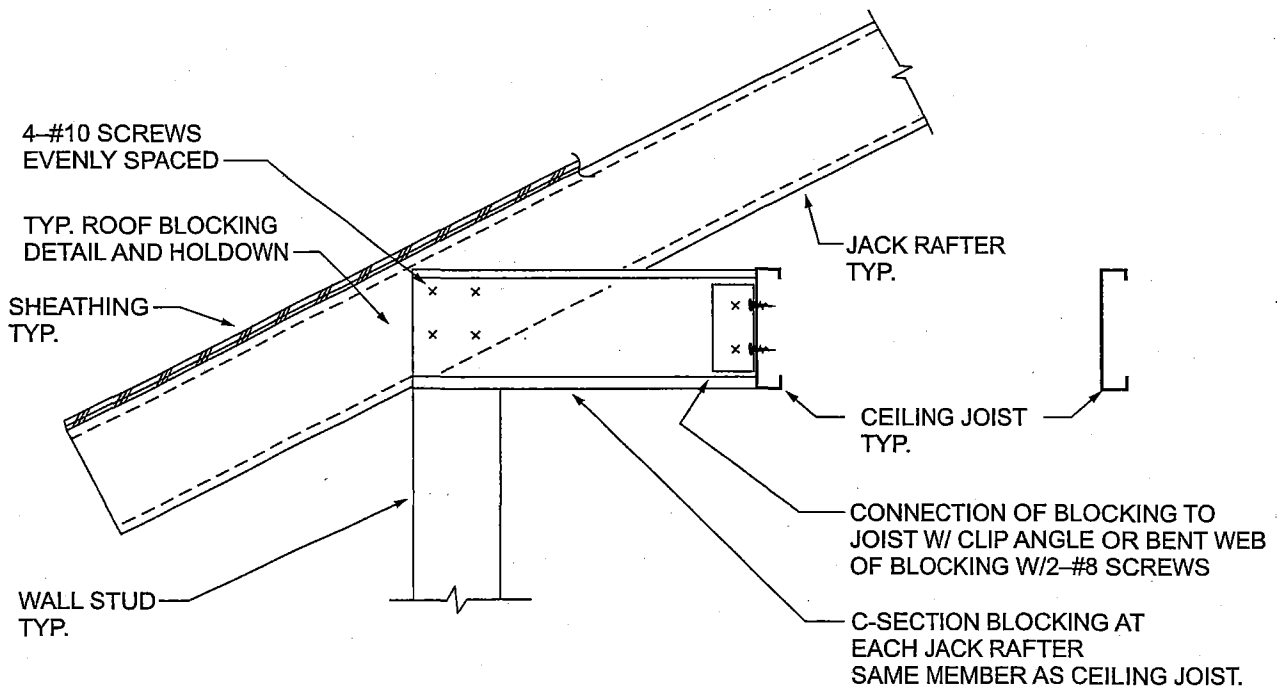
FIGURE R804.3.3.4(1) JACK RAFTER CONNECTION AT EAVE
