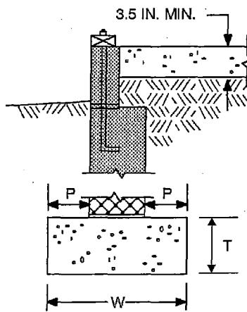
GROUND SUPPORT SLAB WITH MASONRY WALL AND SPREAD FOOTING
