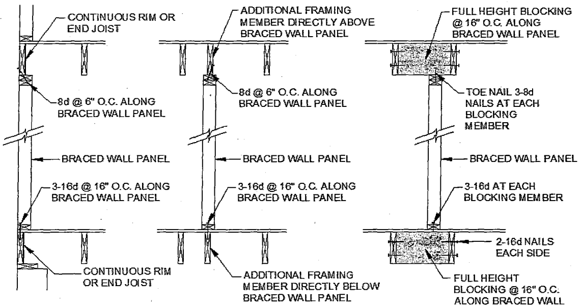
FIGURE R602.10.8(2) BRACED WALL PANEL CONNECTION WHEN PARALLEL TO FLOOR/CEILING FRAMING
