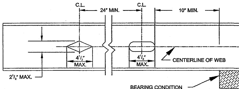
FIGURE R804.2.5.1 WEB HOLES
