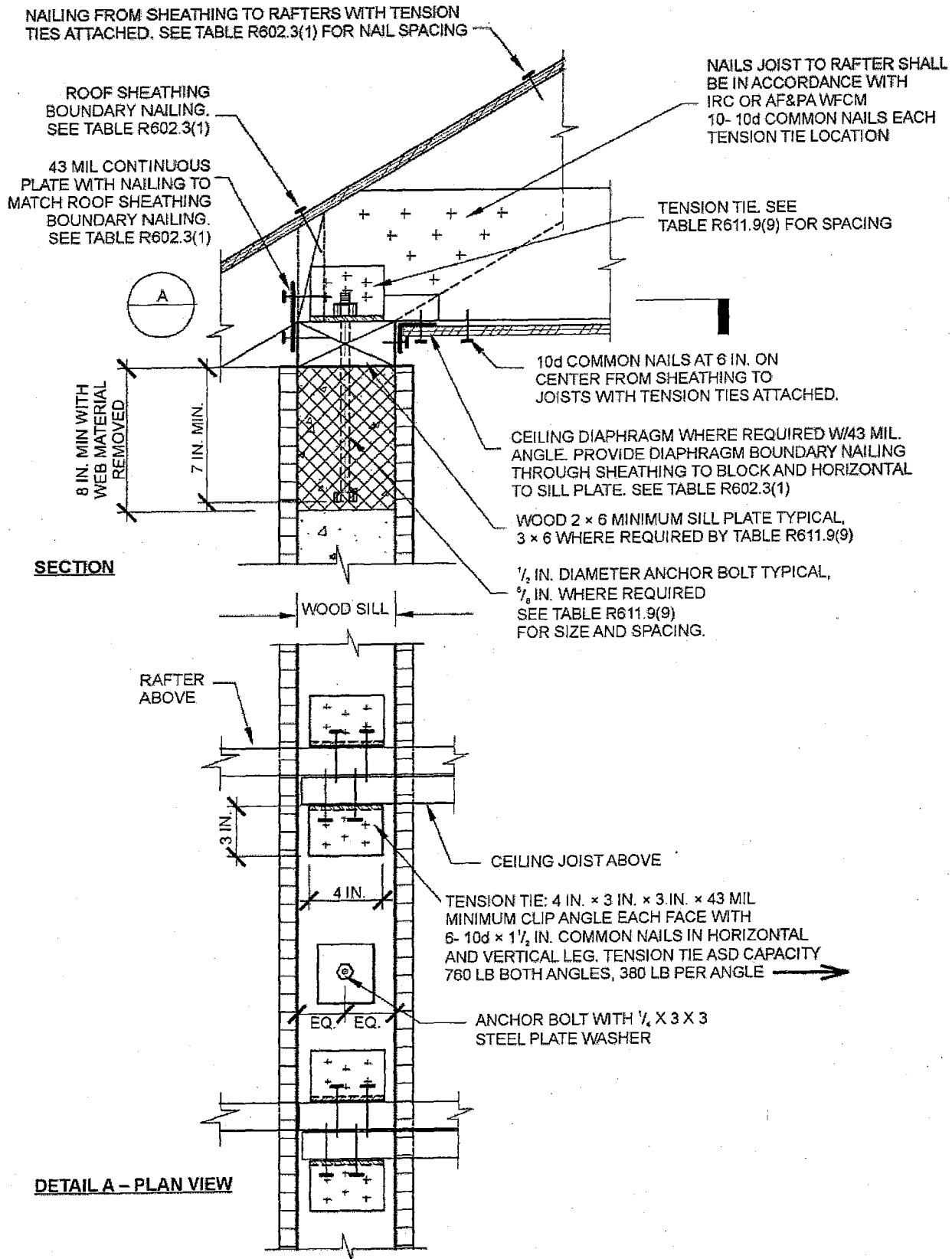
FIGURE R611.9(9) WOOD-FRAMED ROOF TO TOP OF CONCRETE WALL, FRAMING PERPENDICULAR
