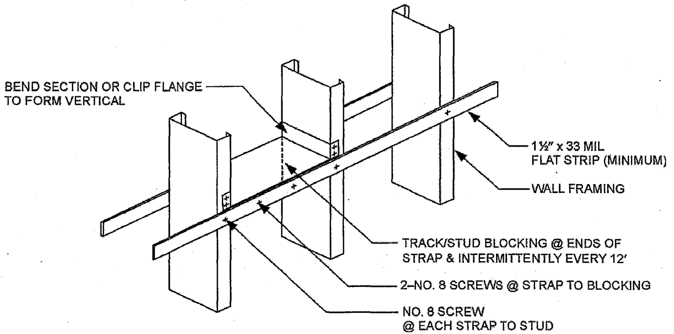
FIGURE R603.3.3(1) STUD BRACING WITH STRAPPING ONLY
