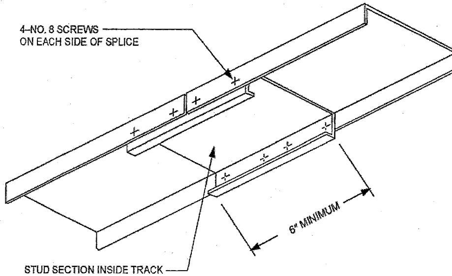
FIGURE R603.3.5 TRACK SPLICE
