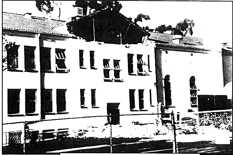
Damage to a private school in the 1994 Northridge earthquake.
