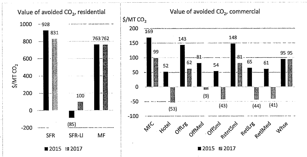
Figure 12 Benefit (or cost) of avoided CO 2 emissions.
