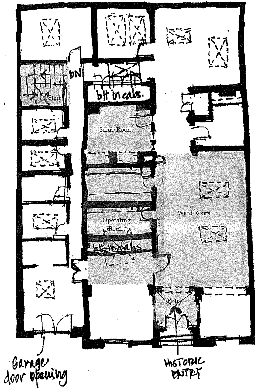
First floor plan; location of character defining features represented by green shading.
