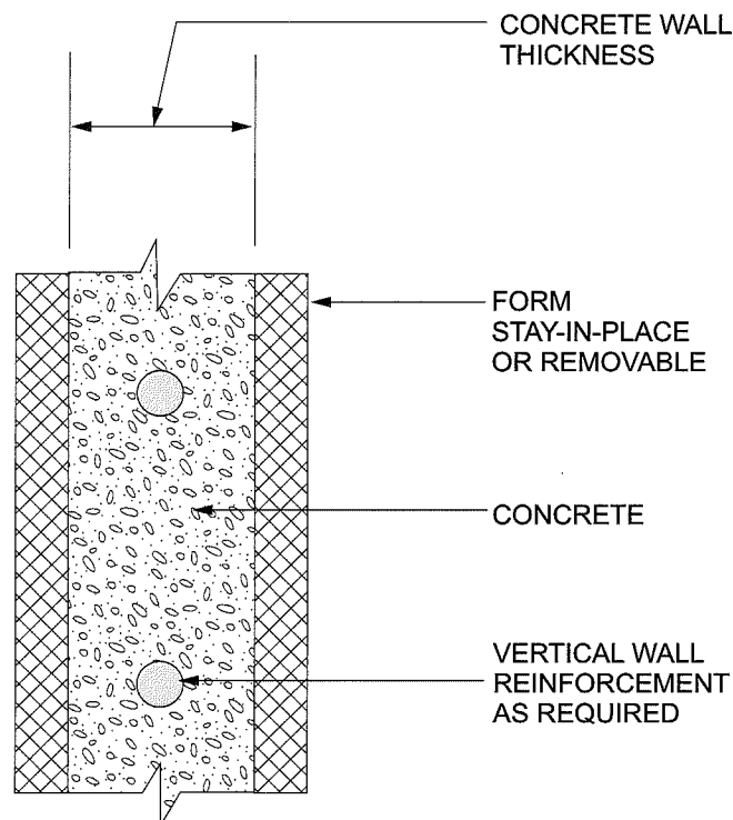
PLAN VIEW
