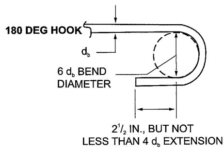
HOOKS FOR REINFORCEMENT IN WALLS AND FOUNDATIONS
