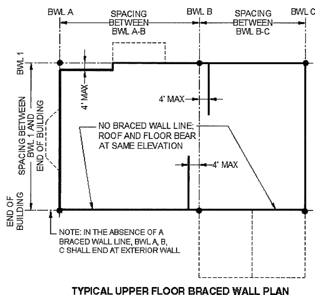
FIGURE R602.10.1.1 BRACED WALL LINES
