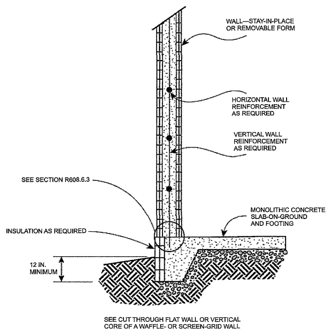
FIGURE R608.6(4)
