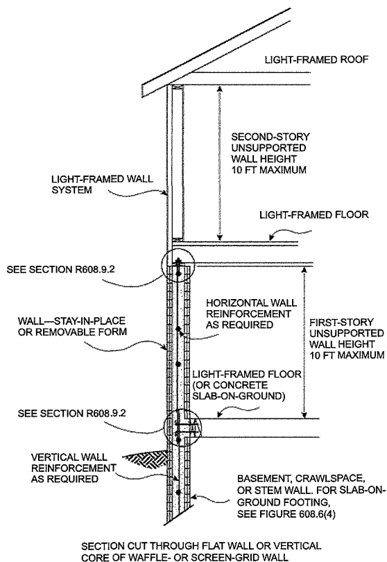
FIGURE R608.6(2)
