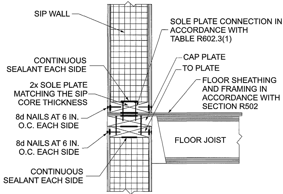
FIGURE R610.5(5) SIP WALL-TO-WALL BALLOON FRAME CONNECTION (I-Joist floor shown for illustration only)
