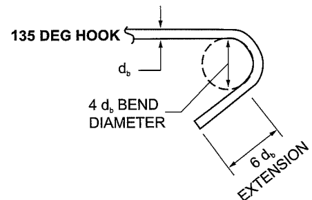
HOOKS FOR STIRRUPS IN LINTELS
