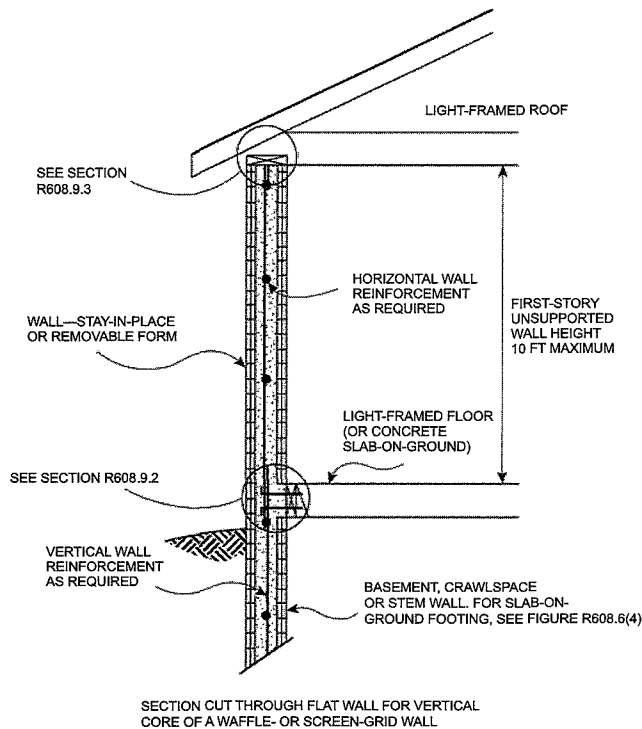
FIGURE R608.6(1)
