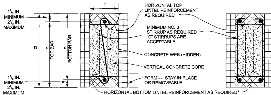
FIGURE R608.8(2) LINTEL FOR FLAT WALLS
