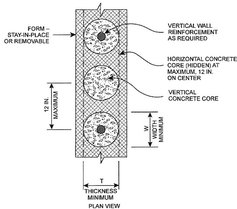
FIGURE R608(2) WAFFLE-GRID WALL SYSTEM
