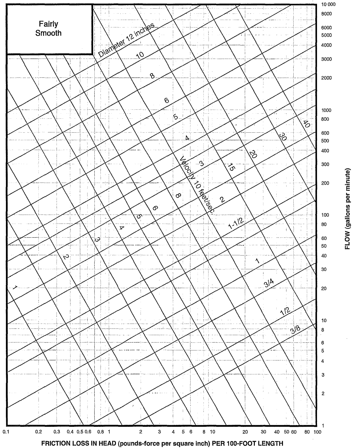
CHART A 105.1(2)
