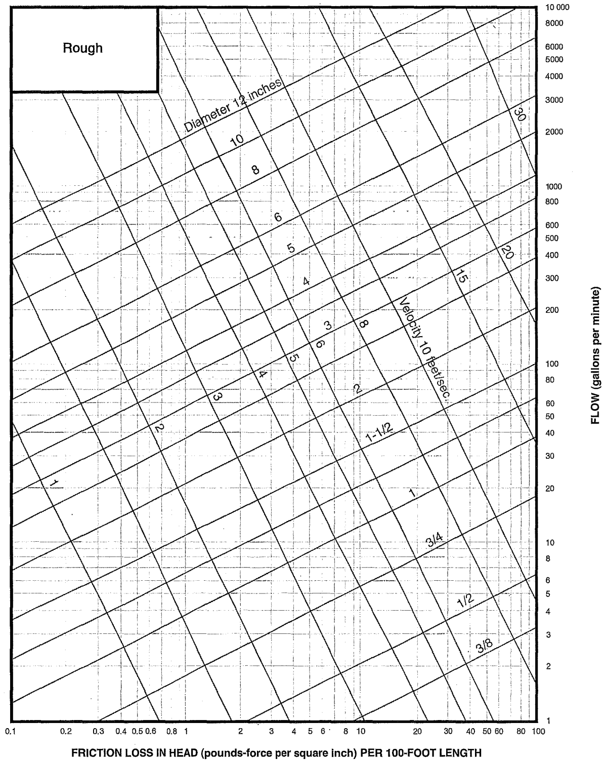
CHART A 105.1(4)
