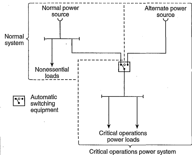
Figure 708.2 Critical Operations Power Systems.
