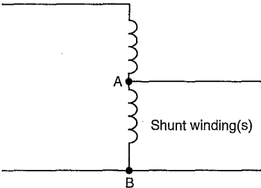
Figure 450.4(A) Autotransformer.
