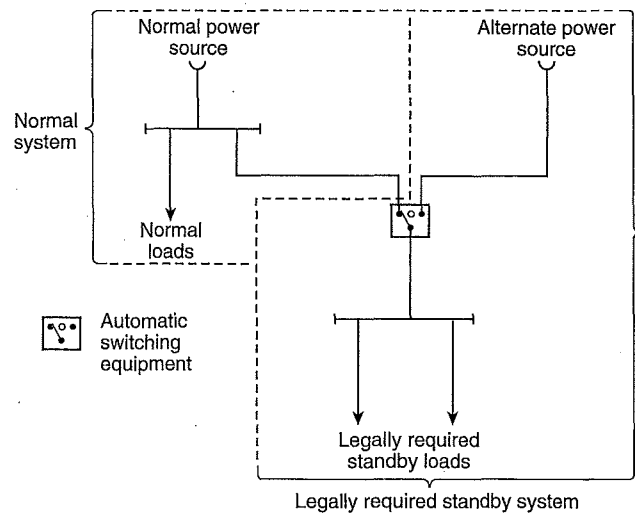
Figure 701.2 Legally Required Standby Systems.
