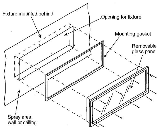
Figure 516.4(C)(3) Example of a Luminaire that is an Integral Part of the Spray Area and is Serviced from Inside the Spray Area. [33:Figure 6.6.3]
