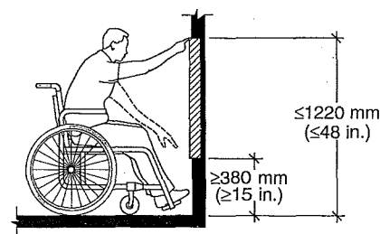
Figure J.6.1 Unobstructed Forward Reach.
