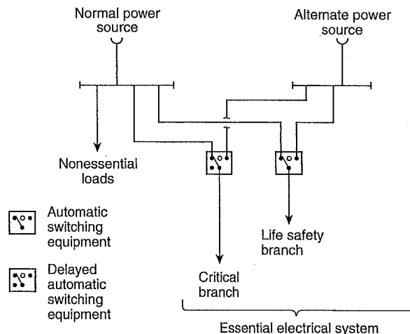
Informational Note Figure 517.41, No. 1 Nursing Home and Limited Health Care Facilities — Minimum Requirement (greater than 150 kVA) for Transfer Switch Arrangement.
