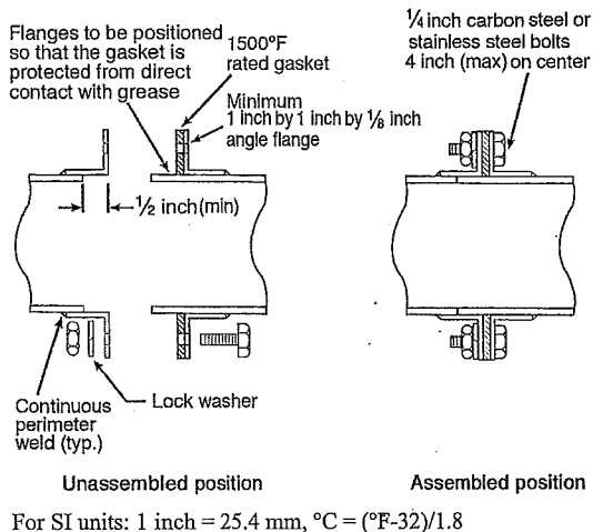
FIGURE 511.1.2(1) TYPICAL SECTION OF DUCT-TO-FAN CONNECTION-BUTT JOINT METHOD [NFPA 96: FIGURE 8.1.3.2(a)]
