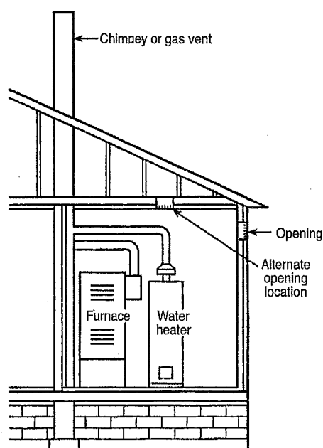
FIGURE 701.6.2 COMBUSTION AIR FROM OUTDOORS THROUGH SINGLE COMBUSTION AIR OPENING [NFPA 54: FIGURE A.9.3.3.2]
