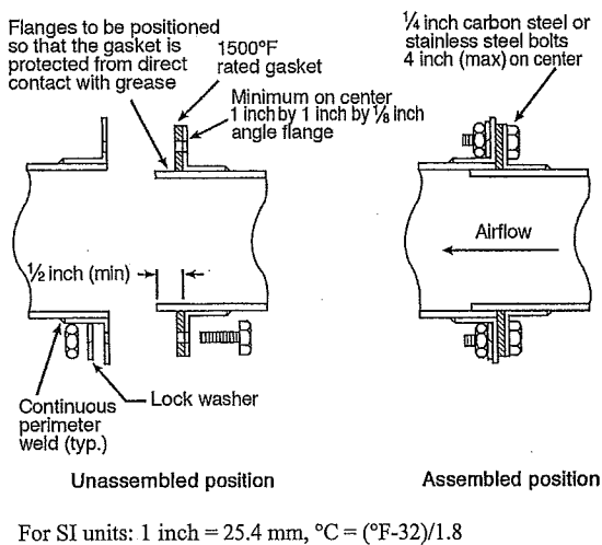
FIGURE 511.1.2(2) TYPICAL SECTION OF DUCT-TO-FAN CONNECTION-OVERLAPPING METHOD [NFPA 96: FIGURE 8.1.3.2(b)]
