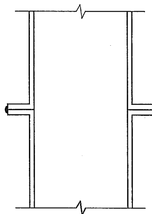
FIGURE 510.5.3.2(3) FLANGE WITH EDGE WELD DUCT CONNECTION [NFPA 96: FIGURE 7.5.5.1(c)]
