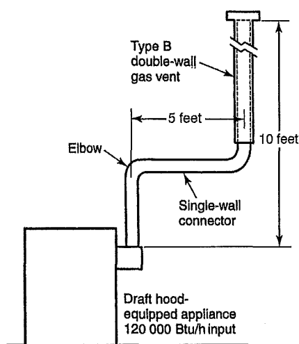
»» FIGURE G 101.3 SINGLE DRAFT HOOD-EQUIPPED APPLIANCE – EXAMPLE 1
