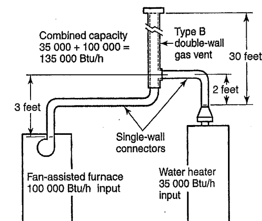
FIGURE G 101.7 COMMON VENTING A DRAFT HOOD-EQUIPPED WATER HEATER WITH A FAN-ASSISTED FURNACE INTO A TYPE B DOUBLE-WALL COMMON VENT – EXAMPLE 5(a)
