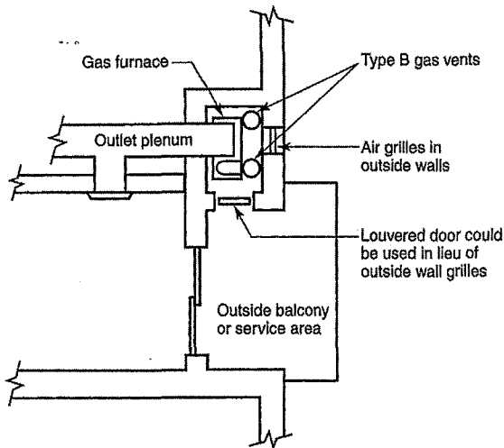
FIGURE 509.6.4.1 PLAN VIEW OF PRACTICAL SEPARATION METHOD FOR MULTISTORY GAS VENTING [NFPA 54: FIGURE A.12.7.4.2]
