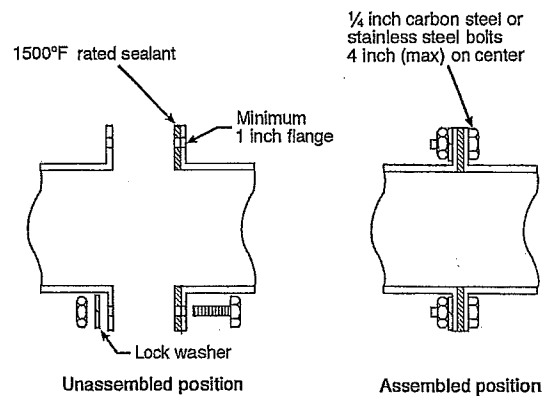
FIGURE 511.1.2(3) TYPICAL SECTION OF DUCT-TO-FAN CONNECTION-SEALANT METHOD [NFPA 96: FIGURE 8.1.3.2(c)]
