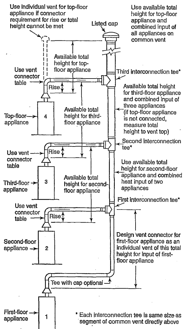
FIGURE 803.2.13 PRINCIPLES OF DESIGN OF MULTISTORY VENTS USING VENT CONNECTOR AND COMMON VENT DESIGN TABLES [NFPA 54: FIGURE F.1(n)]
