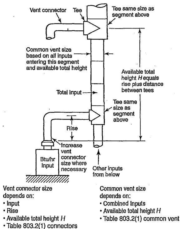
FIGURE F 101.1(13) MULTISTORY GAS VENT DESIGN PROCEDURE FOR EACH SEGMENT OF SYSTEM
