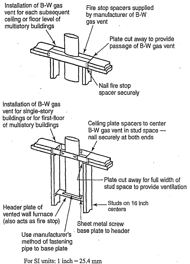
FIGURE 907.1 INSTALLATION OF TYPE B-W GAS VENTS FOR VENTED WALL FURNACES [NFPA 54: FIGURE 10.27.1.3]
