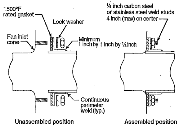
FIGURE 511.1.2(4) TYPICAL SECTION OF DUCT-TO-FAN CONNECTION- DIRECT TO FAN INLET CONE METHOD [NFPA 96: FIGURE 8.1.3.2(d)]
