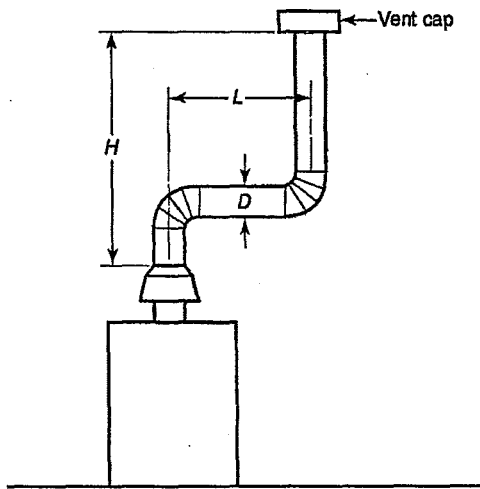
FIGURE F 101.1(5) ASBESTOS CEMENT TYPE B OR SINGLE-WALL METAL VENT SYSTEM SERVING A SINGLE DRAFT HOOD-EQUIPPED APPLIANCE
