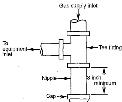
FIGURE 1212.8 METHOD OF INSTALLING A TEE FITTING SEDIMENT TRAP [NFPA 54: FIGURE 9.6.7]
