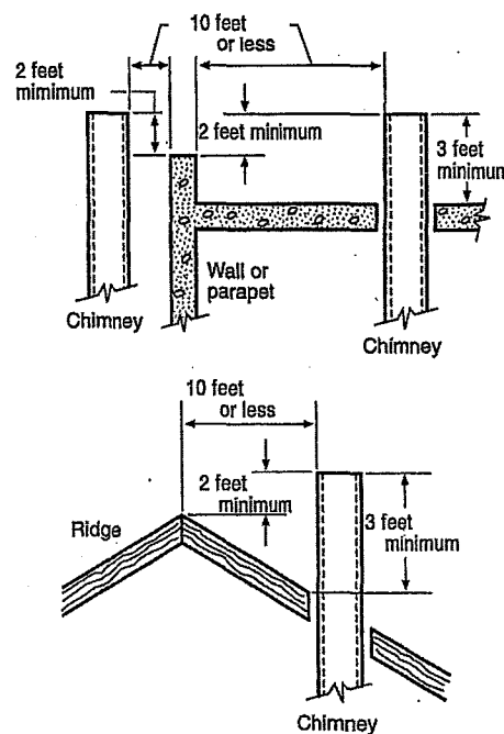
(a) Termination 10 feet or Less from Ridge, Wall, or Parapet
