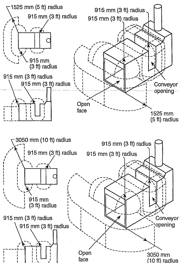
Figure 516.3(D)(2) Class I, Division 2; Class I, Zone 2; Class II, Division 2; or Zone 22 Locations Adjacent to a Closed Top, Open Face, or Open Front Spray Booth or Room.
