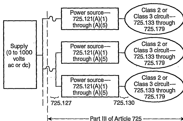
Informational Note Figure 725.121, No. 1 Class 2 and Class 3 Circuits.
