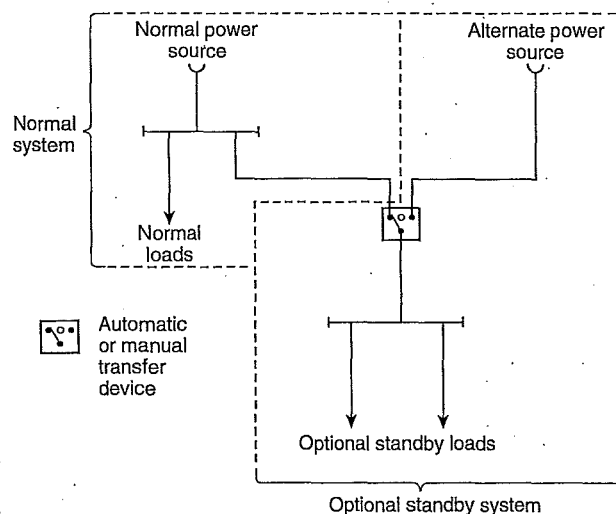
Figure 702.2 Optional Standby Systems.
