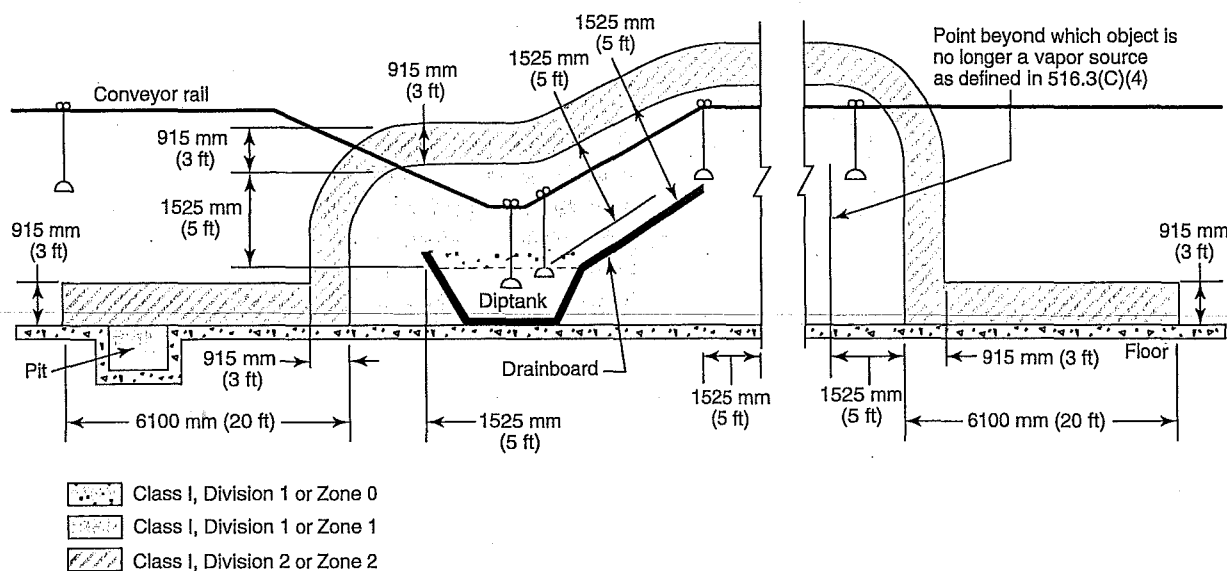
Figure 516.3(D)(6)(a) Electrical Area Classification for Open Dipping and Coating Processes Without Vapor Containment or Ventilation. [34:Figure 6.4(a)]
