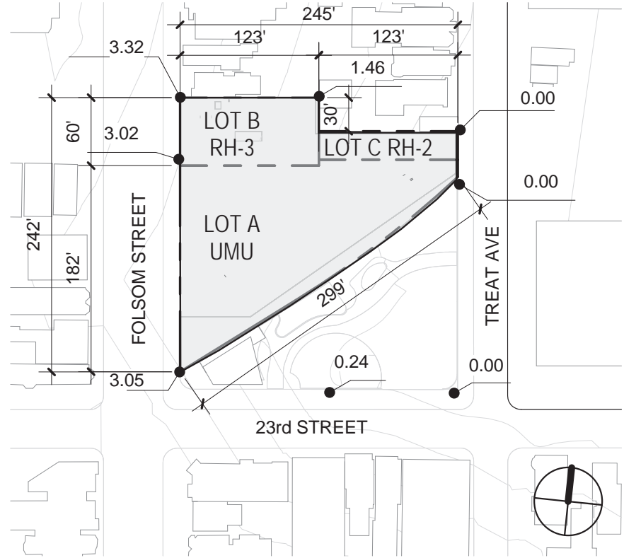
1 SITE PLAN 1" = 120'-0"
