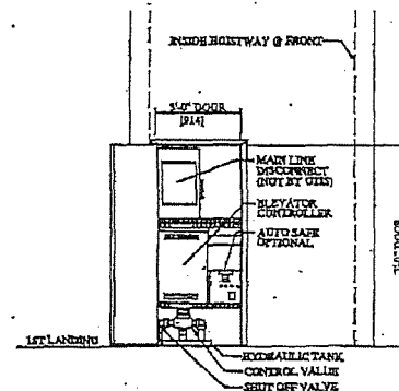
SECTION Q-Q
