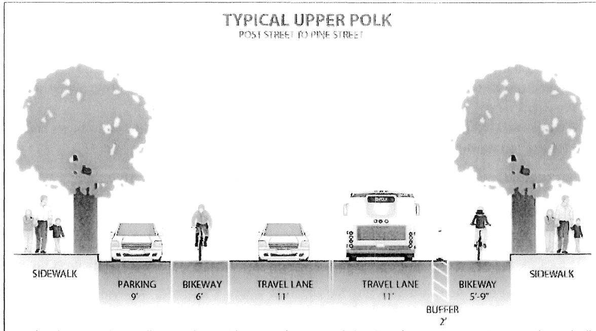
Figure 5 SFMTA Polk Street Lane Improvements Plan
