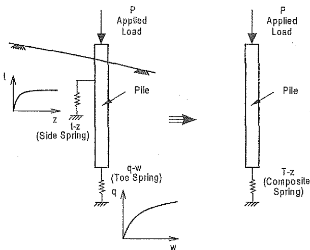
FIGURE 31F-6-1 AXIAL SOIL SPRINGS [6.8]
