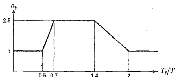
FIGURE 31F-4-9 AMPLIFICATION FACTOR, a_p [4.10]
