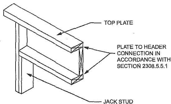
FIGURE 2308.5.5.1(2) ALTERNATIVE SINGLE-MEMBER HEADER WITHOUT CRIPPLE
