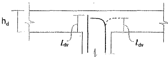
FIGURE 31F-7-9 DEVELOPMENT LENGTH
