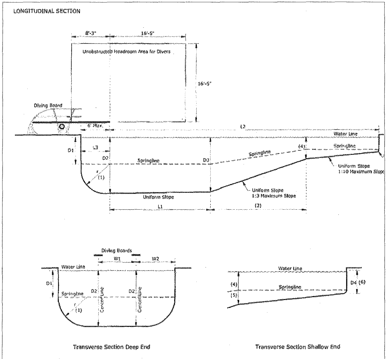
FIGURE 31B-1 DEPTHS AND CLEARANCES FOR POOLS WITH DIVING BOARDS GREATER THAN 30 INCHES (762 mm) ABOVE THE WATER LINE
