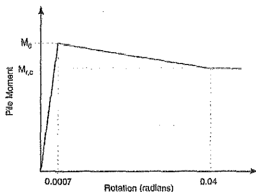
FIGURE 31F-7-12 JOINT ROTATION
