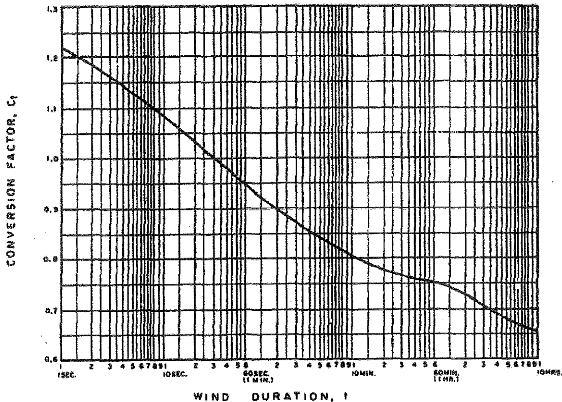
FIGURE 31F-3-1 WIND SPEED CONVERSION FACTOR [3.5]
