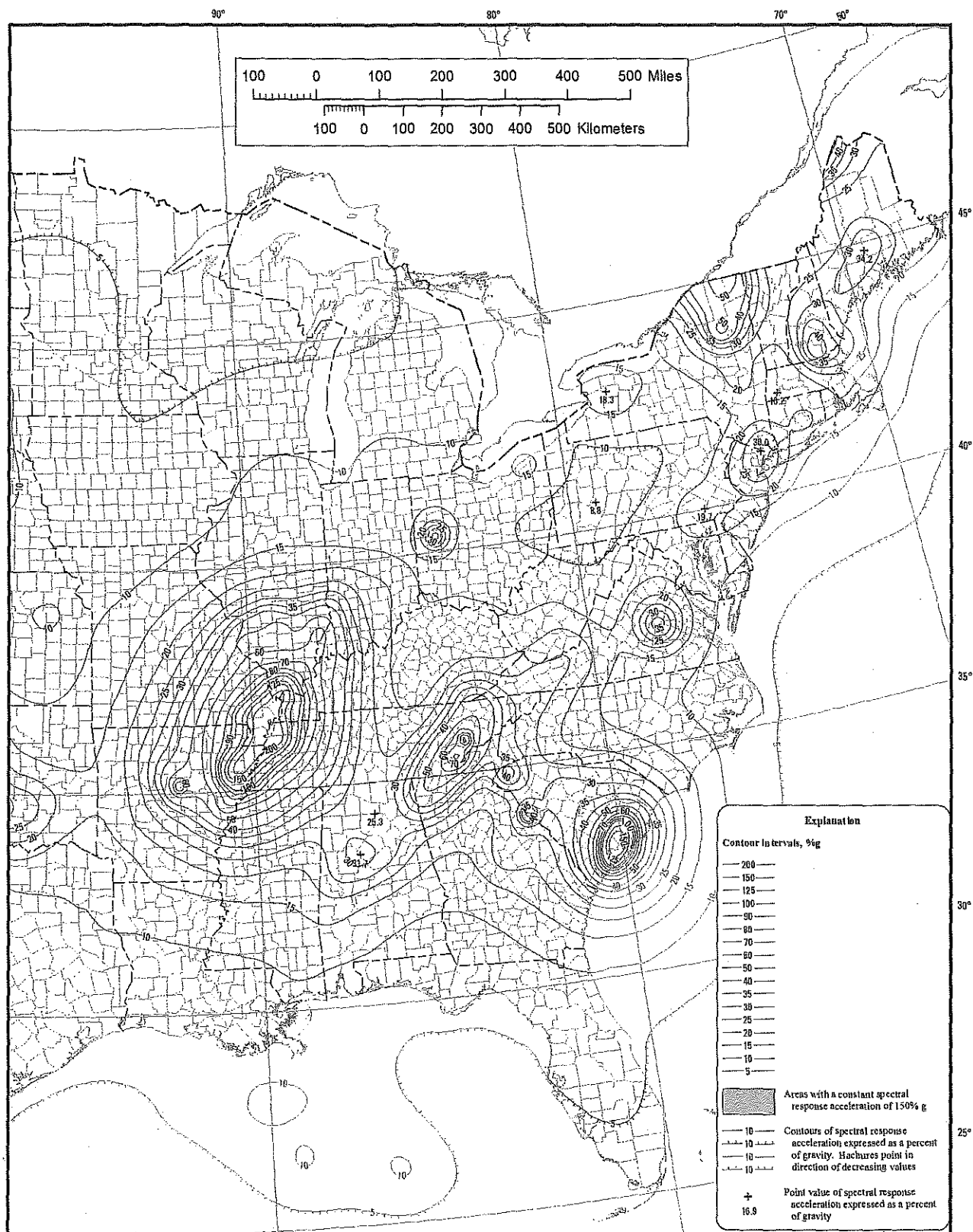
FIGURE 1613.2.1(1)—continued RISK-TARGETED MAXIMUM CONSIDERED EARTHQUAKE ( MCE_R ) GROUND MOTION RESPONSE ACCELERATIONS FOR THE CONTIGUOUS UNITED STATES OF 0.2-SECOND SPECTRAL RESPONSE ACCELERATION (5% OF CRITICAL DAMPING)
