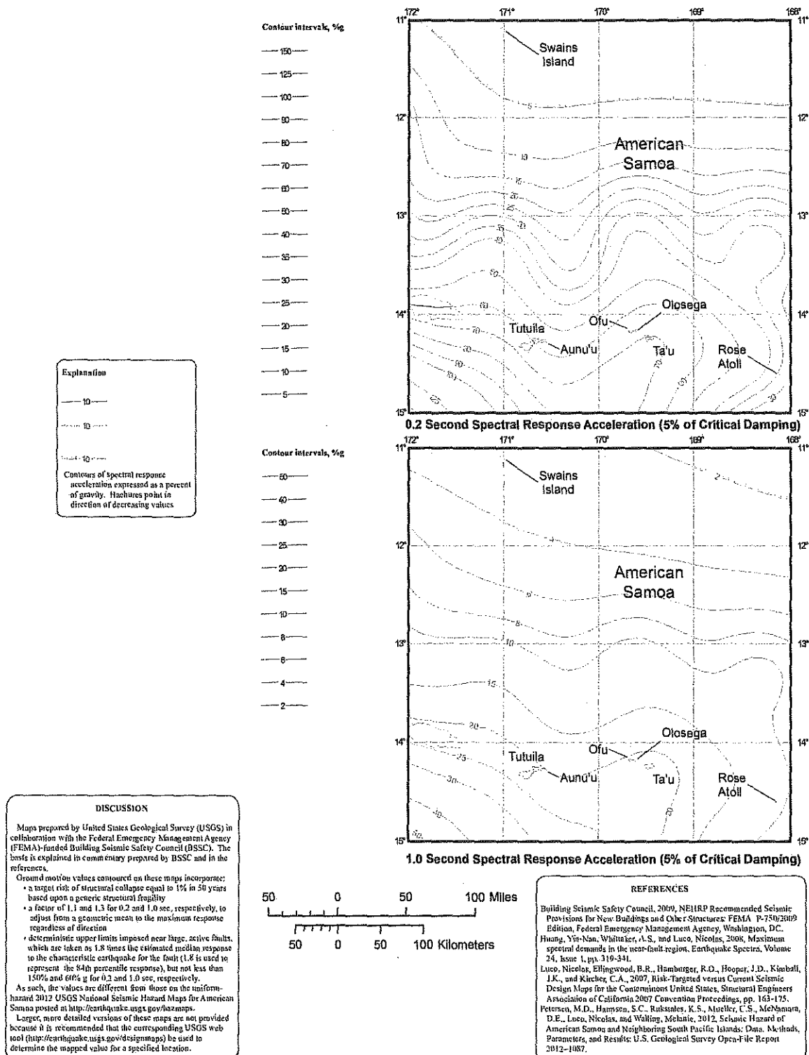
FIGURE 1613.2.1(8) RISK-TARGETED MAXIMUM CONSIDERED EARTHQUAKE (MCE) GROUND MOTION RESPONSE ACCELERATIONS FOR AMERICAN SAMOA OF 0.2- AND 1-SECOND SPECTRAL RESPONSE ACCELERATION (5% OF CRITICAL DAMPING)
