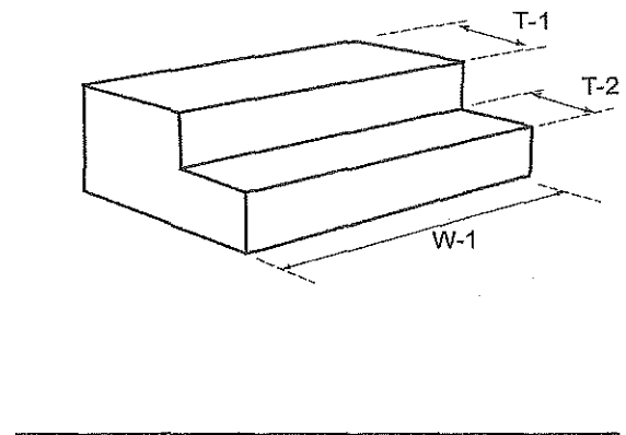
Standard Step
