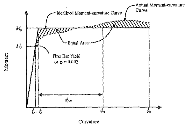
FIGURE 31F-7-5 METHOD B – MOMENT CURVATURE ANALYSIS [7.6]
