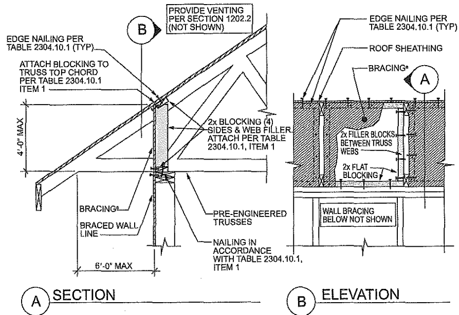
FIGURE 2308.6.7.2(2) BRACED WALL PANEL TOP PLATE CONNECTION
