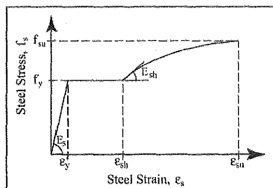
FIGURE 3107F-7-2 STRESS-STRAIN CURVE FOR MILD REINFORCING STEEL OR STRUCTURAL STEEL [7.1]
