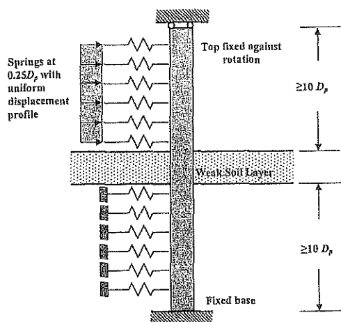
FIGURE 31F-6-2 SLIDING LAYER MODEL [6.8]
