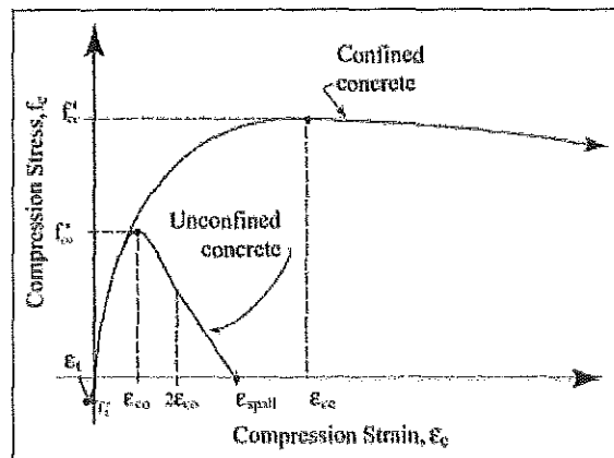
FIGURE 3107F-7-1 STRESS-STRAIN CURVES FOR CONFINED AND UNCONFINED CONCRETE [7.1]
