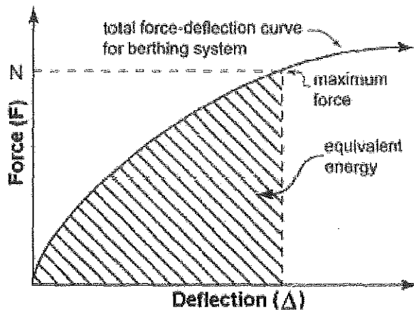
FIGURE 31F-5-5 BERTHING ENERGY CAPACITY
