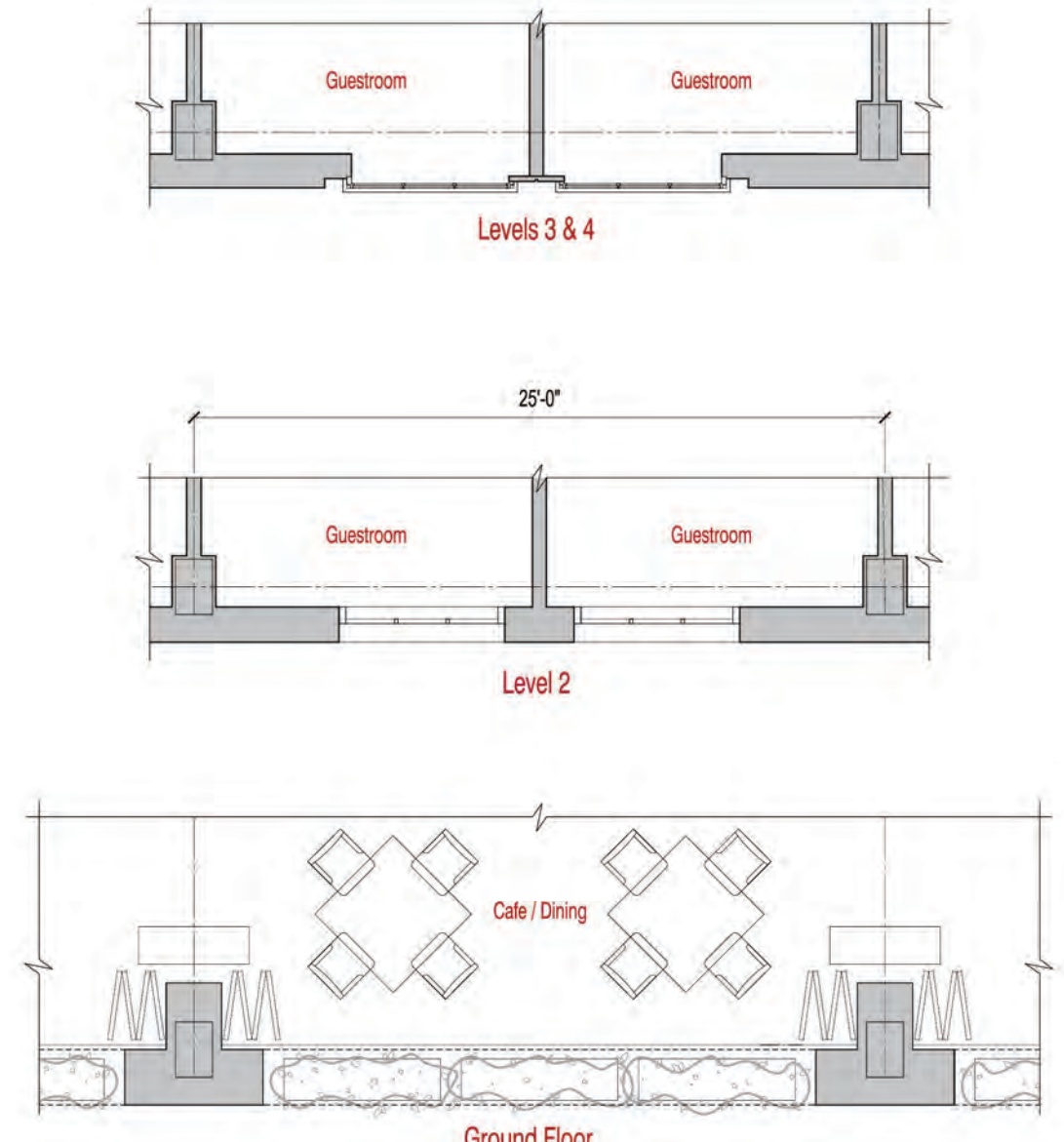
Plan Sections
