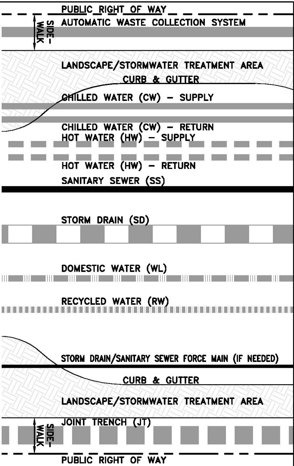
WASTEWATER IN STREETS 1"=10'
